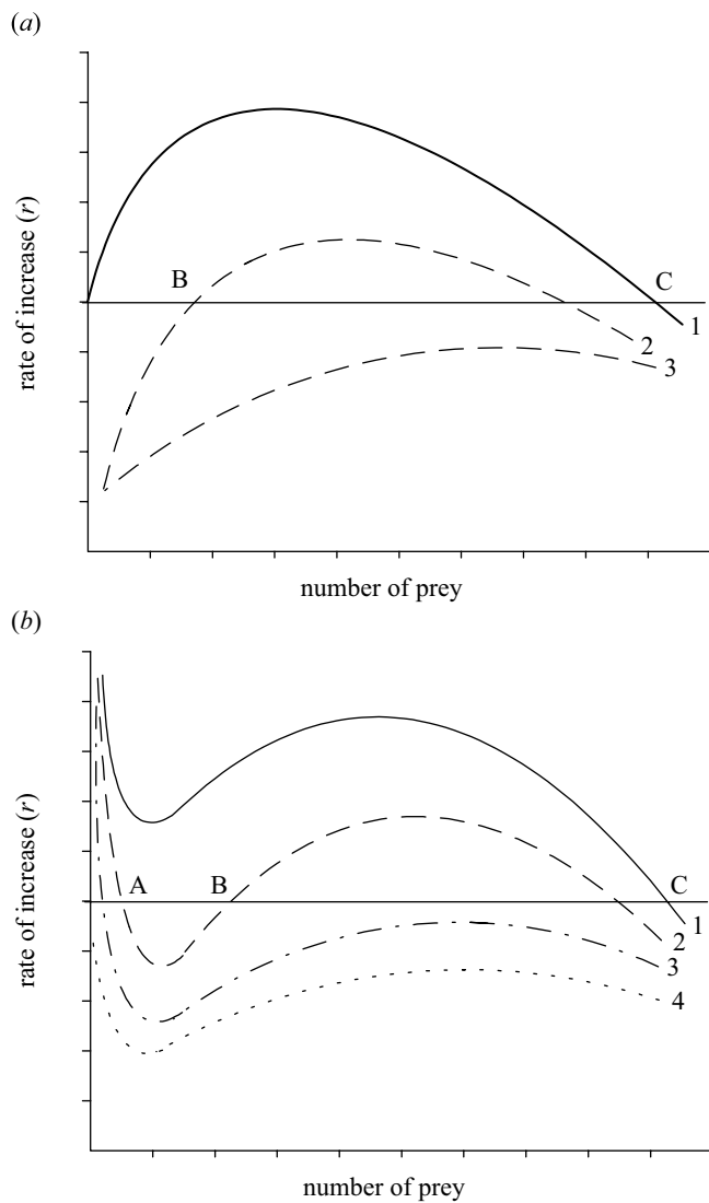
Figure 6. The instantaneous rates of change of the prey population experiencing different levels of (a) type II and (b) type III predation. Point A represents a stable point from regulation by predators, point C a stable point due to regulation from food with predation not regulating, and point B is an unstable threshold. Curves 1–4 represent different intensities of predation: 1, lowest predation level; 4, highest predation level.
