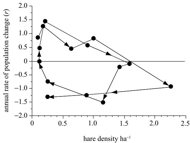
Figure 11. Rate of population increase ( r ) in relation to snowshoe hare density at Kluane, Yukon, from 1986 to 2001. These data comprise the better part of two hare cycles. The rate of increase for the decline phase of the hare cycle follows a different track from that for the increase phase due to time delays in both food and predator effects (Data from Krebs et al. 1999; C. J. Krebs, unpublished data).
