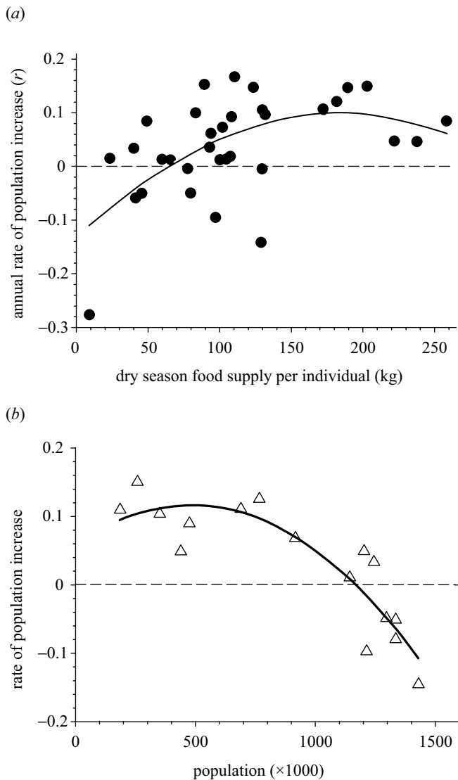
Figure 1. (a) Annual instantaneous rates of increase for the Serengeti wildebeest population as a function of dry season food supply per individual (kg dry season grass individual -1 km -2 ). (b) Wildebeest rate of population increase plotted against population size (data from Mduma et al. 1999).
