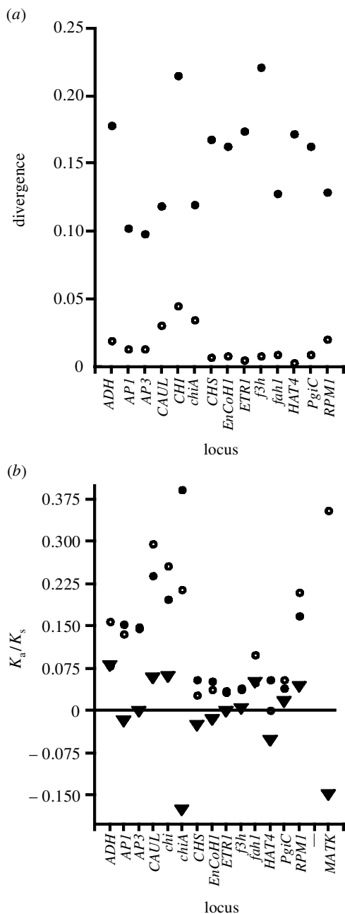
Figure 5. Divergence between Arabidopsis thaliana and A. lyrata for synonymous and non-synonymous sites in 15 nuclear loci. (a) K_a (open circles) and K_s (filled circles) values, and (b) the K_a/K_s ratios estimated for the lineages since the two species separated, as well as the K_a/K_s differences between the two lineages. No A. lyrata result is shown for MATK because it exceeds the maximum value on the y-axis. Arabidopsis thaliana (open circles); A. lyrata (filled circles); A. thaliana – A. lyrata (filled inverted triangles).
