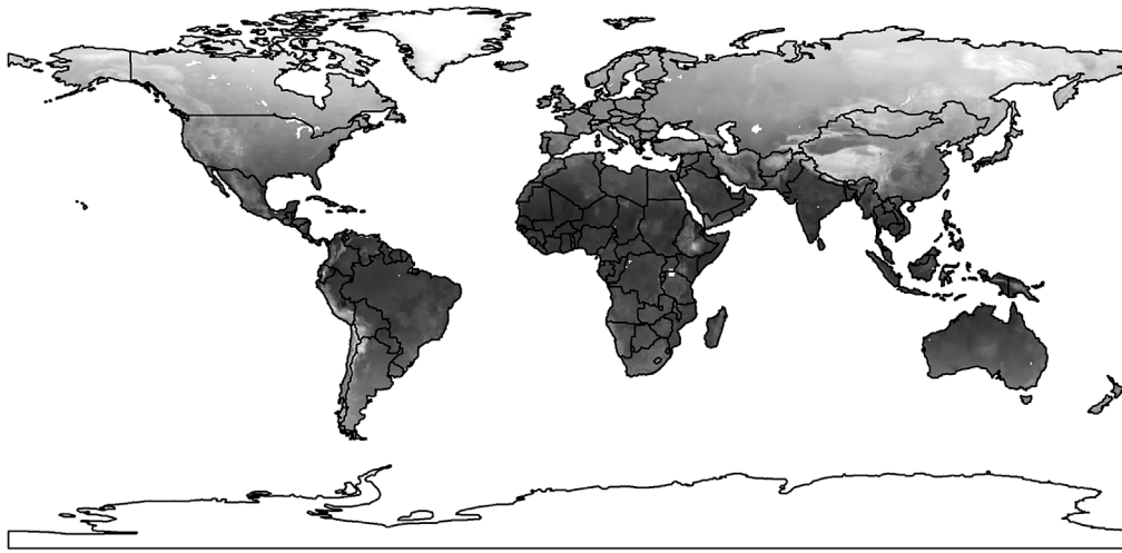
Figure 3. Average surface air temperature obtained from the online Global Ecosystem Database ( http://www.ngdc.noaa.gov/seg/ecco/cdroms/gedii_a/datasets/a03/lc.htm ), between 1931 and 1960, from low (light) to high (dark).
