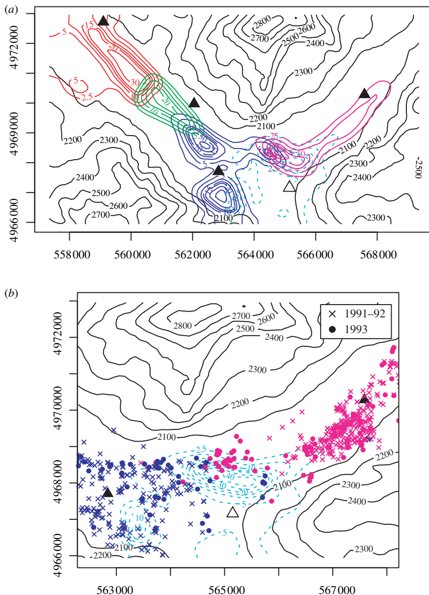
Figure 3. (a) Coloured contour lines show the spatial distribution of home ranges in Lamar Valley predicted by the PA+CA model following loss of the centrally located Norris pack in January 1993. Solid contour lines show the new configuration of home ranges in relation to the former home range of the Norris pack indicated by the dashed light-blue contour lines. Patterns of space-use of the prior to the removal are shown in figure 2b. Black contour lines show topographic relief in metres. The location of the former home range centre of the Norris pack (open triangle) and the locations of the home range centres of the remaining packs (filled triangles) are also shown. (b) Observed changes in space-use by the Soda Butte and Fossil Forest packs following the loss of the Norris pack in January 1993. As in (a), the dashed light-blue contour lines show the former home range of the Norris pack. Coloured points show the relocations of individuals in the neighbouring Soda Butte (pink) and Fossil Forest (blue) packs prior to (crosses) and following (filled circles) the loss of the Norris pack. As predicted by the model (a), the Soda Butte and Fossil Forest packs expand their territories into the former Norris home range following the loss of the Norris pack focusing their movements on the prey-rich mesic grassland north of the former Norris home range centre (open triangle).
