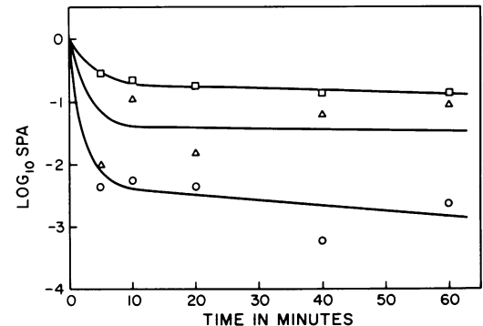
FIG. 9. Kinetics of aggregation of reovirus at pH 3.0. Initial single particle concentrations: □, 4.6 \times 10^{10} ; Δ, 1.8 \times 10^{10} ; ○, 1.8 \times 10^9 .
