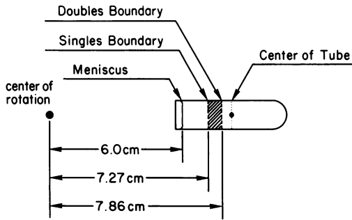
FIG. 1. This diagram gives the basic measurements for the SPA test. Although any rotor can be used, the values given here are for the Beckman SW50.1 rotor utilizing 0.5- by 2-inch (1.27 by 5.08 cm) tubes. The terms "singles boundary" and "doubles boundary" refer to the distance traveled by single and double particles, respectively, from the meniscus of the fluid under the influence of the centrifugal force.
