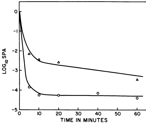
FIG. 5. Kinetics of aggregation of poliovirus at pH 3.0 in 0.05 M glycine-HCl buffer. Initial single particle concentrations: △, 7 × 10 9 ; ○, 7 × 10 10 .
