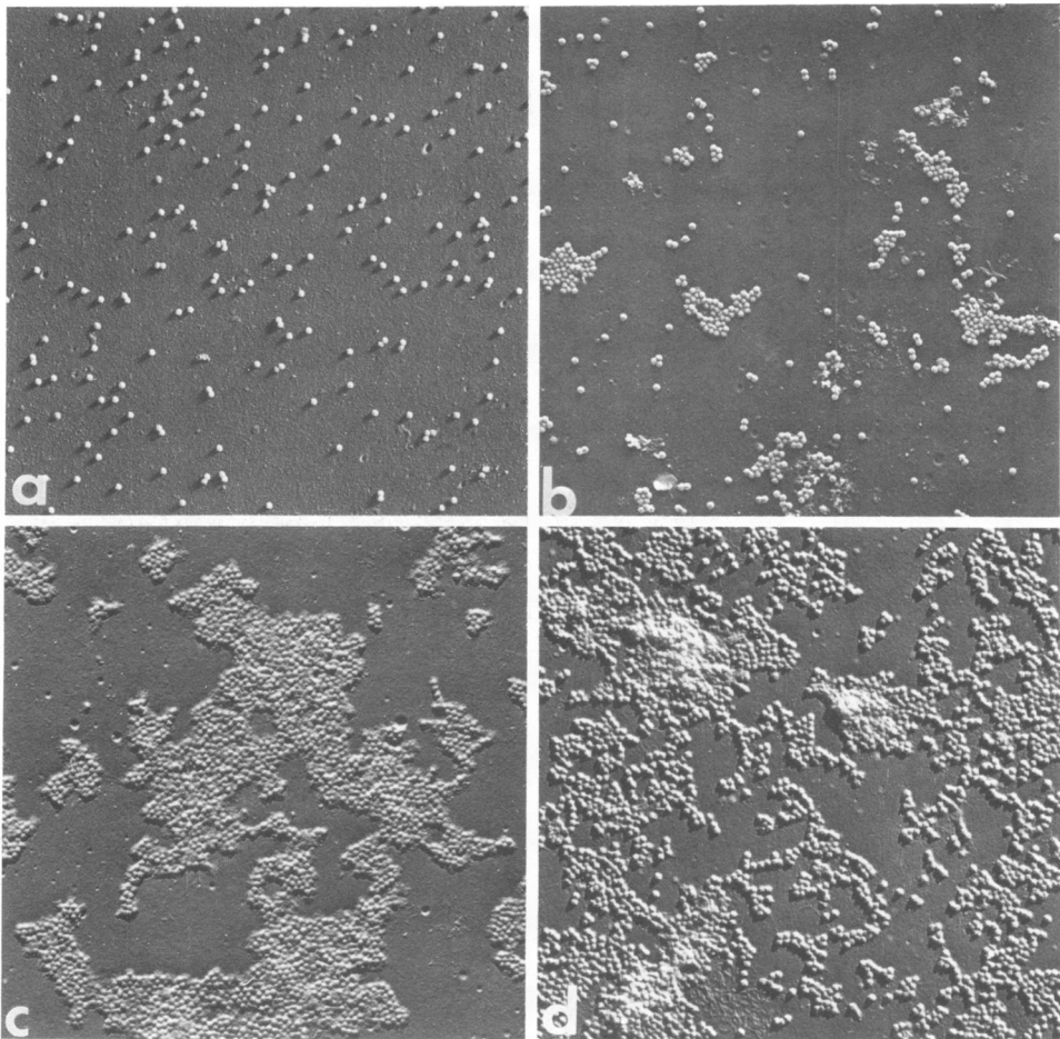
FIG. 6. Reovirus stock at 2 \times 10^{10} virions/ml diluted (a) 200-fold in PBS and (b) 10-fold in distilled water, allowed to remain at room temperature for 2 h, and then further diluted 20-fold in PBS. Both were prepared for electron microscope examination by the spin-down method. (c) Stock at 4.6 \times 10^{11} virions/ml diluted in 0.05 M acetate at pH 5.0. (d) Same stock as (c) diluted in 0.05 M glycine-HCl, pH 3.0. Particles in (c) and (d) were collected by the kinetic attachment method. \times 8,500 .
