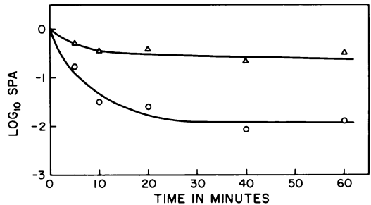
FIG. 8. Kinetics of aggregation of reovirus at pH 5.0. Initial single particle concentrations: Δ, 4.6 \times 10^{10} ; ○, 10^{10} .
