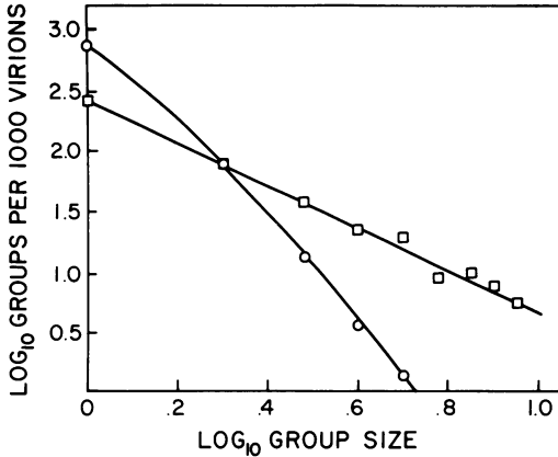
FIG. 7. Dual-log plot of the frequency of aggregates in the stock reovirus preparation of Fig. 6 (○) and after extensive aggregation induced by dilution in water (□), as shown in Fig. 6b. The slope of each line is a quantitative measure of the aggregation, and the difference in slope between the two lines is a relative measure of the aggregation produced by the dilution in water.
