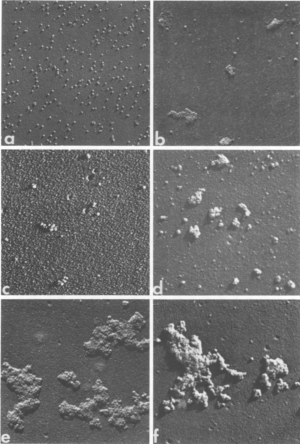
FIG. 2. A poliovirus stock concentrate at 7 \times 10^{11} virions/ml was diluted 10-fold in (a) PBS; (b) distilled water; (c) 0.01 M \text{CaCl}_2 ; (d) 0.05 M phosphate, pH 6.0; (e) 0.05 M acetate, pH 5.0; and (f) 0.05 M glycine-HCl, pH 3.0. All were prepared for electron microscope examination by the kinetic attachment method. (a) \times 24,800 ; (b)-(f) \times 29,000 .
