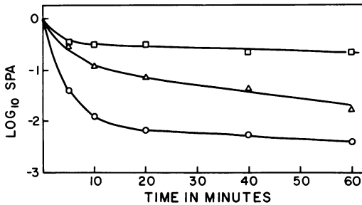
FIG. 4. Kinetics of aggregation of poliovirus at pH 5.0 in 0.05 M acetate buffer. Initial single particle concentrations: □, 1.5 × 10 10 ; △, 3 × 10 10 ; ○, 1.5 × 10 11 .
