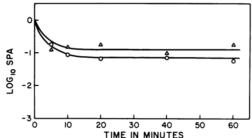
FIG. 3. Kinetics of aggregation of poliovirus at pH 6.0 in 0.05 M phosphate buffer as determined by the SPA test. Initial single particle concentrations: \Delta , 1.4 \times 10^{10} ; \circ , 7 \times 10^{10} .
