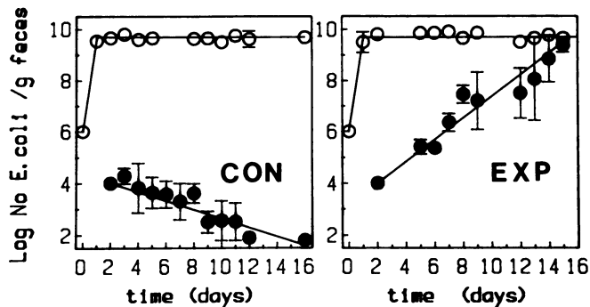
FIG. 1. Competition between two isogenic strains of E. coli in gnotobiotic mice drinking pure water (CON) or 2 \mu g of streptomycin per ml of water (EXP). Germfree mice were inoculated on day zero with 10^6 plasmid-free E. coli EM0 bacteria (○) and on day 2 with 10^4 plasmid pYD1-bearing bacteria (●). Each point represents six groups (CON) or two groups (EXP) of three mice each. Curves in panel CON were calculated with the mathematical model given in the text, with the following numerical values: \rho = 0.08 per h; \mu_s = \mu_r = 1.66 per h; K_{s_s} = 0.0009 g/liter; K_{s_r} = 0.001 g/liter; L_i = 0.005 g/liter; Y = 10^{12} bacteria per g. Equation 6 replaces equation 1 for calculation of the curves in panel EXP, and the numerical value of AB was set at 0.06 per h.
