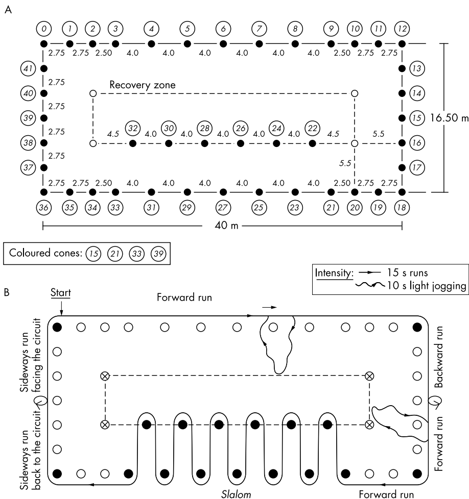
Figure 1 The Bangsbo soccer field test circuit. (A) Circuit dimensions. The length and width of the circuit correspond to that of the penalty area of a soccer pitch. The recovery zone is delimited by four small cones at the corners and wooden batters on the field. Cones 15 and 39 correspond to running direction changes, and cones 21 and 33 to the beginning and end of the slalom. They should be of different colour to be easily identified. The four cones at the area corners (0, 12, 18, and 36) and the slalom cones (21–33) must be at least 1.2 m high. The others can be small cones. (B) The test lasts 16.5 minutes, during which players alternate between 40 15 second bouts of high intensity exercise and 10 second low intensity exercise jogs. During the high intensity periods, subjects follow the 160 m circuit, running 40 m forward, 8.25 m backwards, 95.25 m forward and through a 120° angle slalom, 8.25 m sideways while facing away from the centre of the circuit, and 8.25 m sideways while facing the centre of the circuit. During the low intensity periods, players jog to the centre of the circuit and back to the last cone marked position they reached at the end of the previous high intensity period. If the sound signal stops them during the slalom, the low jogging is performed towards the next slalom cone and back to the last cone they reached before the signal. The test performance is the distance covered during the 40 periods of high intensity running.
