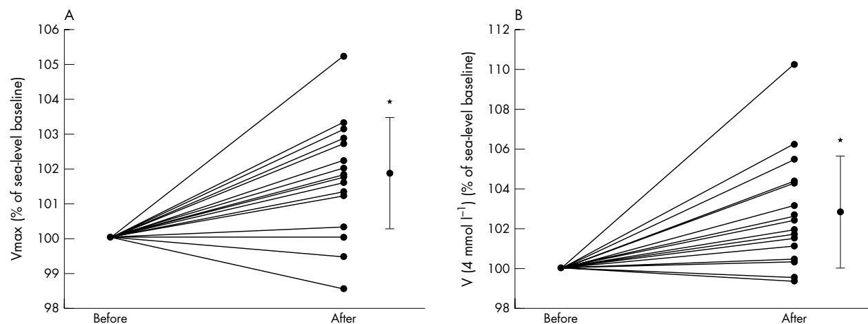
Figure 3 Changes in maximal performance and in performance at a 4 \text{ mmol l}^{-1} lactate concentration in an incremental swimming test. The data are presented as per cent sea level baseline values. Individual values and mean values and standard deviation are shown. *Indicates significantly different from sea level baseline ( p < 0.001 ). V, velocity.
