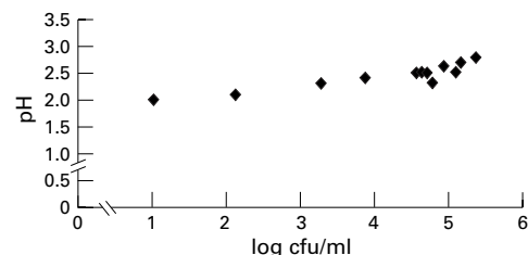
Figure 2 pH in universal containers at the end of the experiment versus number of surviving H pylori (starting pH=2 in all experiments).
