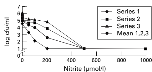
Figure 1 Antibacterial activity of nitrite against H pylori at pH 2 after 30 minutes' exposure. Experiments were carried out in triplicate (series 1, 2, and 3). No survival was detected at concentrations of nitrite ≥500 µmol/l.
