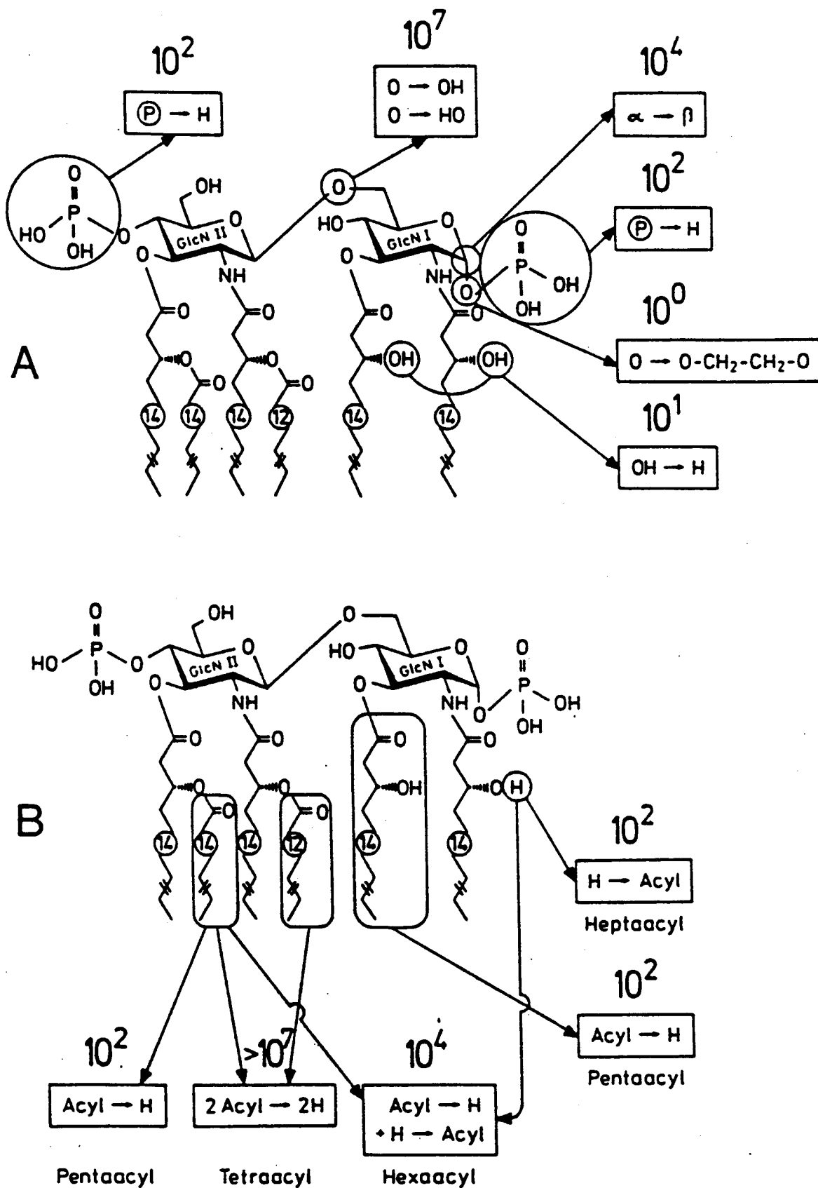
FIG. 3. Schematic representation of lipid A structure-activity relationships. Shown are chemical changes of the E. coli lipid A structure and the factor by which the structure generated is less active than lipid A as determined by their ability to activate the production of mononuclear cell peptide mediators. (A) Modifications of the hydrophilic region of lipid A. (B) Modifications of the hydrophobic region of lipid A. Reprinted from reference 316 with permission of the publisher.
