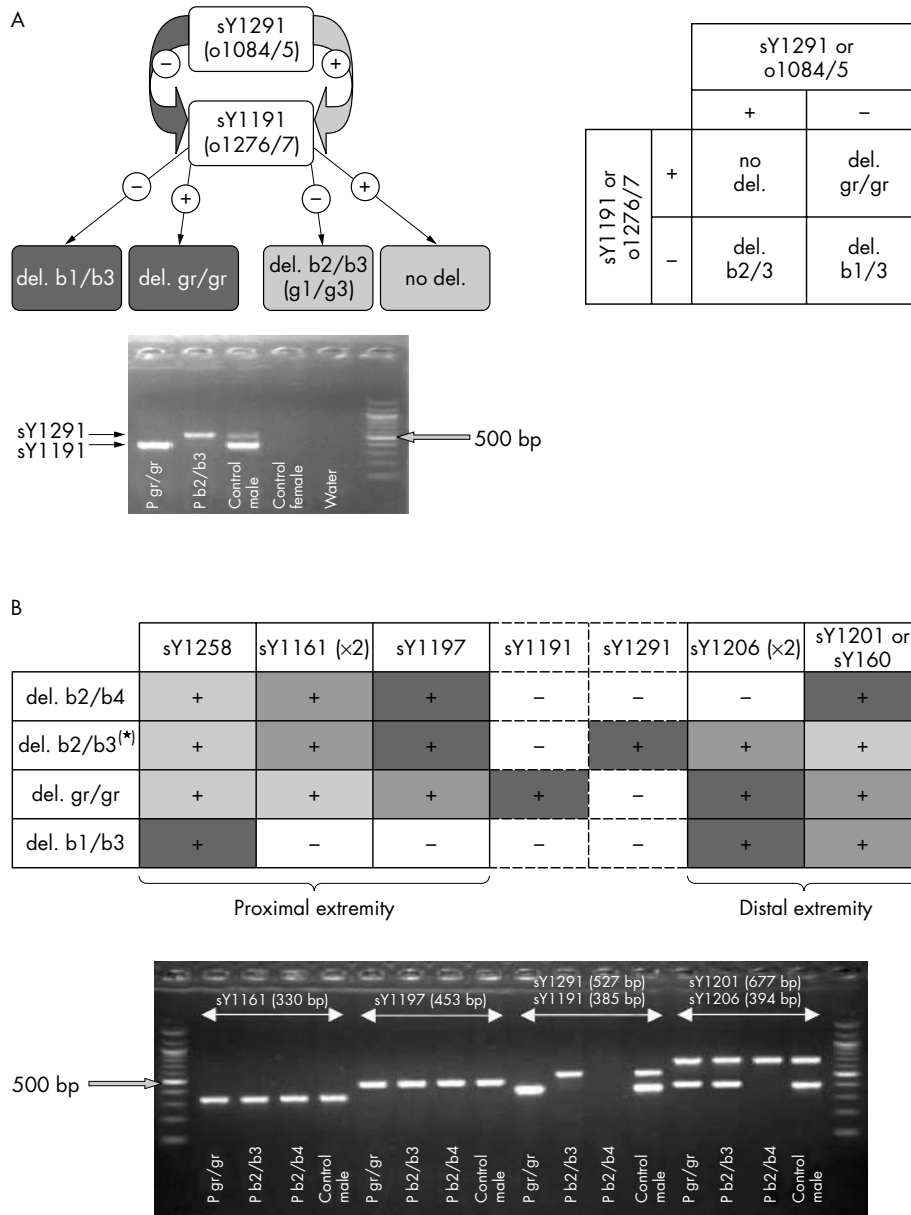
Figure 1 Schematic representation of the proposed two step analysis for the detection of partial AZFc deletions. (A) the first step based on a PCR duplex with sY1191/1291 (alternatively, with o1084/5 and o1276/7) shows the four different possible outcomes of the analysis: b1/b3, gr/gr, b2/b3 (or u3-gr/gr or g1/g3), or absence of deletion; (B) the second step defines the breakpoints of the deletions.
