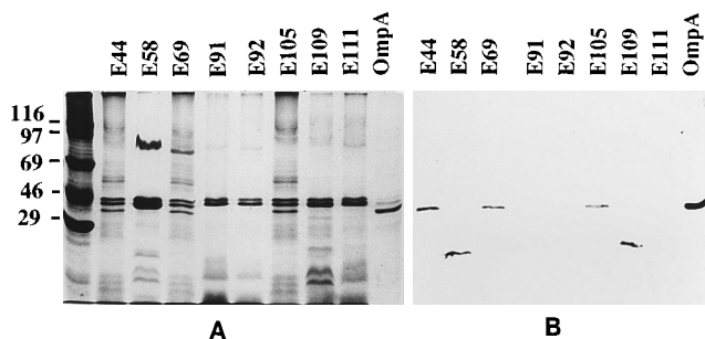
FIG. 1. SDS-PAGE (A) and anti-OmpA antibody Western blot (B) of outer membrane proteins of OmpA + and OmpA - strains. The 3% LDS-soluble membrane proteins of different bacteria were separated on SDS-10% polyacrylamide gels and stained with Coomassie blue. A duplicate gel was transferred to a nitrocellulose sheet and immunoblotted with anti-OmpA antibody as described in the text. The molecular mass markers (in kilodaltons) are indicated on the left.
