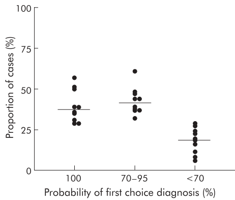
Figure 2 Diagnostic confidence of first choice diagnoses. The median prevalence of biopsy specimens considered to be pathognomonic was 39% (range 29–57%), the median prevalence thought to be pathognomonic or made with high confidence (>70% likelihood) was 82% (range 73–94%), and the median prevalence for diagnoses with low confidence (<70% likelihood) was 18% (range 6–27%).
