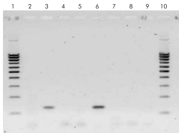
Figure 1 Chlamydomphila pneumoniae nested PCR. Lanes 1 and 10, 100 bp DNA ladder; lanes 2–5, clinical samples; lane 6, positive control; lanes 7–9, negative controls. Lanes 3 and 6 show positive 128 bp PCR products for C pneumoniae .
