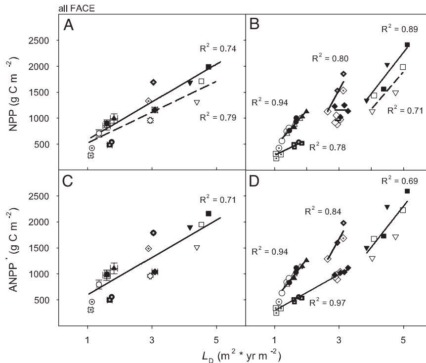
Fig. 3. NPP (A and B) and ANPP' (C and D) as functions of leaf-area duration ( L_D ; m^2 \times yr m^{-2} ) at the four FACE sites. Regressions were fitted to the combined individual treatment-year data from the four sites, but treatment averages for all years within a site (with 1 SE) are shown (A and C). The treatment-year data for each site and the within-site regression fits are shown in B and D. Symbols for species: Duke FACE; P. taeda (circles for unfertilized, up triangles for fertilized), ORNL-FACE; L. styraciflua (diamonds), POP-EUROFACE; P. alba (inverted triangles), P. nigra (squares), Populus euramericana (diamonds with dot), AspenFACE; Populus tremuloides (circles with dot), P. tremuloides/Betula papyrifera (squares with dot), with filled symbols representing elevated [CO_2] . For cases in which current and elevated [CO_2] have different responses (in A and B), dashed and solid lines are used for these treatments, respectively.
