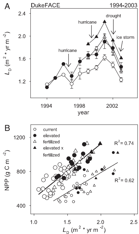
Fig. 2. Annual dynamics of leaf area duration at Duke FACE under current and elevated [CO 2 ] ( L_D ; m^2 \times yr m^{-2} ) (A) and NPP ( g C m^{-2} ) as a function of L_D under wet and dry conditions, as defined by growing season precipitation minus potential evapotranspiration (B). Smaller symbols in B indicate data from dry conditions; relationships were not significantly different between current and elevated [CO 2 ] under wet or dry conditions.
