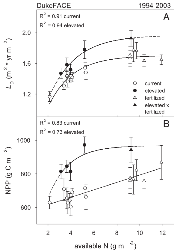
Fig. 1. Five-year (fertilized plots) to 10-year (unfertilized plots) plot-level average leaf area duration ( L_D ; m^2 \times yr m^{-2} ) (A) and NPP ( g C m^{-2} ) (B) as functions of soil-available N under current and elevated atmospheric [CO 2 ] in Duke FACE. Error bars indicate 1 SE among years.
