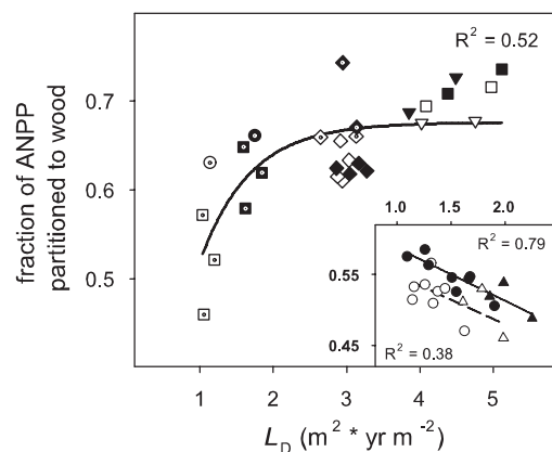
Fig. 4. The fraction of ANPP' partitioned to wood as a function of leaf area duration ( L_D ; m^2 \times yr m^{-2} ) at the four FACE sites. Duke FACE data are shown in Inset. Symbols and lines are as in Fig. 3.
