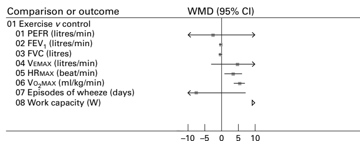
Figure 2 Overall meta-analytical results. Mean value for each outcome is indicated by a square box with the line through it representing the 95% confidence interval (CI). Mean values left of the zero effect line (0) favour control and values on the right favour physical training, except for negative outcomes (where a decrease in the outcome is "good"—for example, episodes of wheeze and maximum heart rate) where mean values left of the zero effect line favour training. A weighted mean difference (WMD) is allocated for each study, which is a method of the meta-analysis used to combine measures on continuous scales. PEFR, peak expiratory flow rate; FEV 1 , forced expiratory volume in one second; FVC, forced vital capacity; HR MAX , maximum heart rate.
