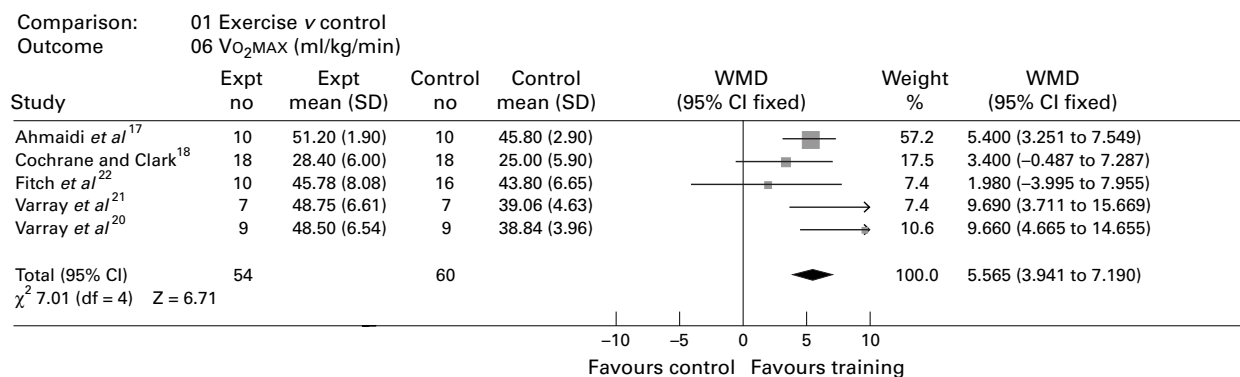
Figure 1 Details of VO 2 MAX (ml/kg/min) outcome. The mean value for each trial is indicated by a square box with the line through it representing the 95% confidence interval (CI). Mean values left of the zero effect line (0) favour control and values on the right favour physical training. The solid diamond indicates the overall mean effect that physical training has on VO 2 MAX. A percentage weighting (Weight %), which is dependent on the precision and sample size of the estimation of the mean value for each randomised controlled trial, is allocated to each study. The \chi^2 (7.01) and the degrees of freedom (df = 4) values at the bottom left give a measure of heterogeneity of the combined results that contributed towards the overall mean result for VO 2 MAX. The Z statistic (6.71) indicates the level of significance for the overall result.
