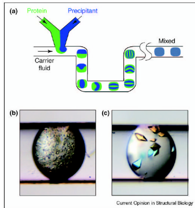
Figure 6. Control of mixing can lead to control of nucleation in protein crystallization. (a) Schematic illustration of the plug-based microfluidic setup for studying the effect of mixing on the nucleation of protein crystals. Mixing by chaotic advection is illustrated. Microphotographs showing an example of the effect of (b) slow chaotic mixing and (c) fast chaotic mixing on protein crystallization under otherwise identical conditions. The diameter of the receiving capillary is 200 \mu\text{m} .
