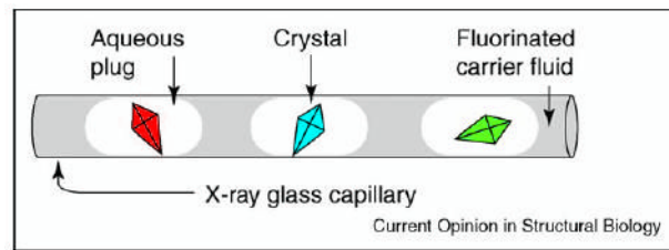
Figure 1. Schematic illustration of protein crystals in aqueous plugs surrounded by fluorinated carrier fluid inside a glass capillary.
