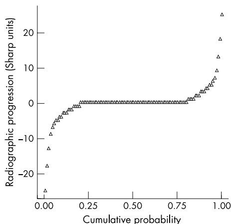
Figure 2 The entire group in reality shows no progression, but there is random measurement error (films scored with the time sequence concealed). The mean change score is 0 (95% CI -1.06 to 1.06).
