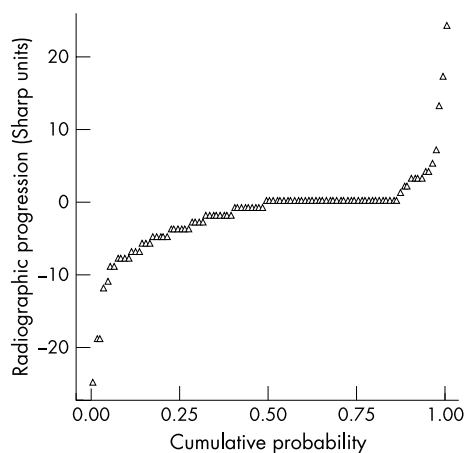
Figure 4. Forty per cent of the cases showing true repair combined with measurement error, by randomly matching the putative true repair scores with putative error scores. The mean change score is -1.7 (95% CI -2.9 to -0.52 ).
