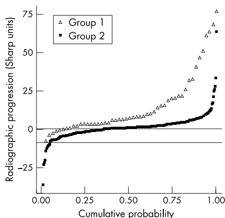
Figure 1 Probability plot of change scores of radiographic damage of two drugs. The x axis shows the cumulative probability and the y axis the actual values. Every single observation is plotted in the curve. The horizontal lines represent a possible binomial cut off point (change of 0 and change of -7).
