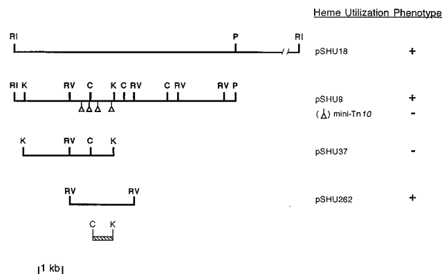
FIG. 1. Partial restriction enzyme map and mini-Tn10 insertional analysis of heme utilization subclones. Open triangles indicate transposon insertion sites which abolish heme iron uptake. The 800-bp ClaI-KpnI probe is shown as a hatched box. The restriction sites shown are ClaI (C), EcoRI (RI), EcoRV (RV), KpnI (K), and PstI (P).
