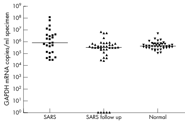
Figure 2 Glyceraldehyde-3-phosphate dehydrogenase (GAPDH) mRNA copies/ml in specimens from severe acute respiratory syndrome (SARS) coronavirus positive patients, follow up specimens, and apparently normal subjects. The median in each group of subjects is indicated by the black horizontal line.
