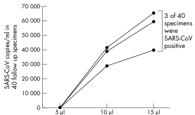
Figure 3 Severe acute respiratory syndrome coronavirus (SARS-CoV) copies/ml in 40 follow up specimens when 5 \mu l, 10 \mu l, and 15 \mu l aliquots of cDNA were used in the quantitative reverse transcriptase polymerase chain reaction assay.
