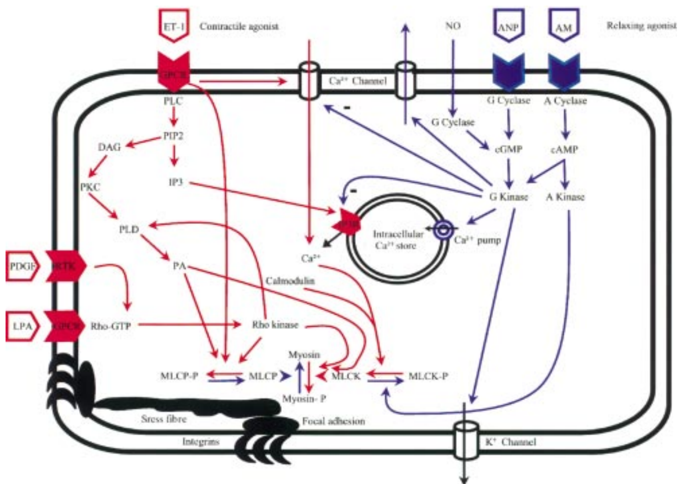
Figure 2 Schematic representation of intracellular contractile and relaxation mechanisms in hepatic stellate cells. It should be noted that most of the pathways have been described in smooth muscle cells but not all mechanisms have been proved to exist in stellate cells. Pathways for contraction are marked in red whereas blue represents relaxation pathways. AM, adrenomedullin; ANP, atrial natriuretic peptide; DAG, diacylglycerol; ET-1, endothelin 1; GPCR, G protein coupled receptor; IP 3 , inositol 1,4,5-trisphosphate; LPA, lysophosphatidic acid; NO, nitric oxide; MLCK, myosin light chain kinase; MLCP, myosin light chain phosphatase; PIP 2 , phosphatidylinositol 4,5-bisphosphate; PLC, phospholipase C; PLD, phospholipase D; PKC, protein kinase C; RTK, receptor tyrosine kinase.
