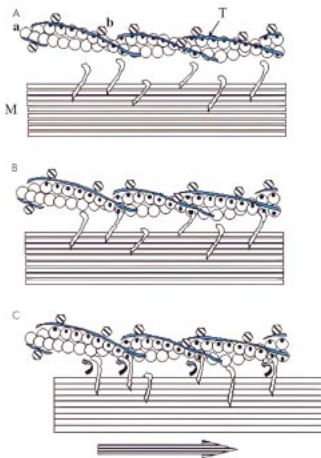
Figure 1 (A) Thin actin filament (a) and thick myosin filament (M) at rest, with tropomyosin (T) covering the myosin binding site and binding proteins with tropomyosin (b). In skeletal muscle, b is troponin; in smooth muscle it is likely to be calponin or caldesmon. (B) Activation of actomyosin: tropomyosin moves from myosin binding sites on actin in two stages—in skeletal muscle, stage 1 is caused by calcium binding to troponin while in smooth muscle stage 1 can be caused by myosin phosphorylation but that is not obligatory. In both cases initial myosin binding causes cooperative conformational changes in stage 2 to fully expose the actin binding sites for myosin. (C) Resulting actomyosin ATPase gives energy for a conformational change in myosin that moves the thick filament relative to the actin thin filament.
