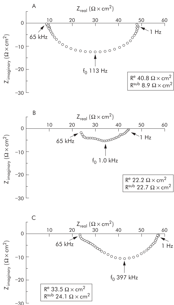
Figure 3 Original impedance locus plots of human sigmoid colon. (A) Control. (B) Crohn's disease (CD) before tumour necrosis factor \alpha (TNF- \alpha ) antibody treatment. (C) CD after TNF- \alpha antibody treatment. Z_{\text{real}} gives the ohmic component and Z_{\text{imaginary}} the reactive component of the complex impedance. Intersections between the semi circle and X axis at low and high frequencies represent R^t and R^{\text{sub}} respectively ( R^t - R^{\text{sub}} = R^e ). R^e , epithelial electrical wall resistance; R^{\text{sub}} , subepithelial electrical wall resistance; R^t , transmural wall resistance.
