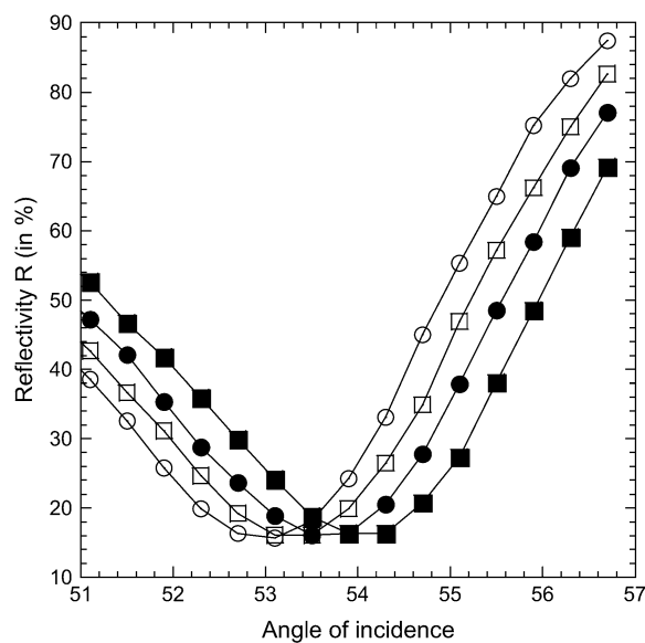
FIGURE 2 Reflectivity as a function of the angle of incidence for different temperatures ( left to right , T = 25, 35, 45, and 55^\circ\text{C} ). The variation of temperature produces a translation of the SPR resonance curve ( \sim 0.04^\circ/\text{C} ) without modification of the sensitivity. The experimental angle of incidence is generally chosen at 55^\circ \pm 1^\circ for a reflectivity close to 30%.
