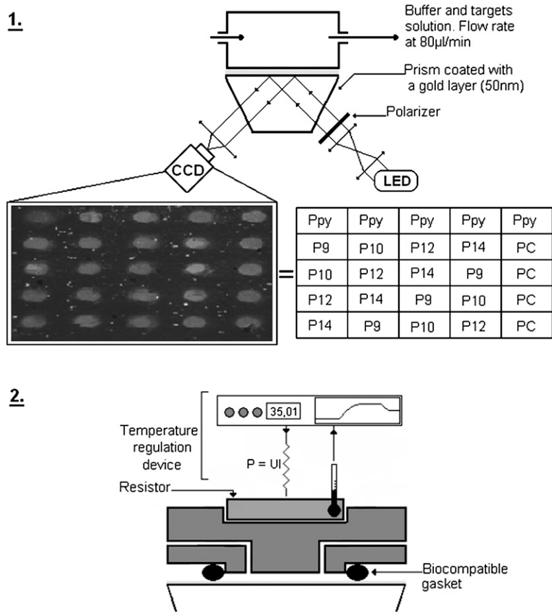
FIGURE 1 (1) Experimental set-up is composed of a LED as the light source ( \lambda = 635 \text{ nm} ). The light is polarized in TE or TM mode by a polarizer and it illuminates the functionalized gold layer in contact with the heating flow cell. Reflectivity changes of each spot are followed using a CCD camera monitored by a LabView interface. The inset table gives the positions of each probe sequence grafted onto the gold surface. (2) Schematic representation of the temperature control device. A resistor, integrated in a stainless steel flow cell, is used to heat the cell solution. The electric power of the resistor is regulated in real time to control the variation of the temperature in the cell.
