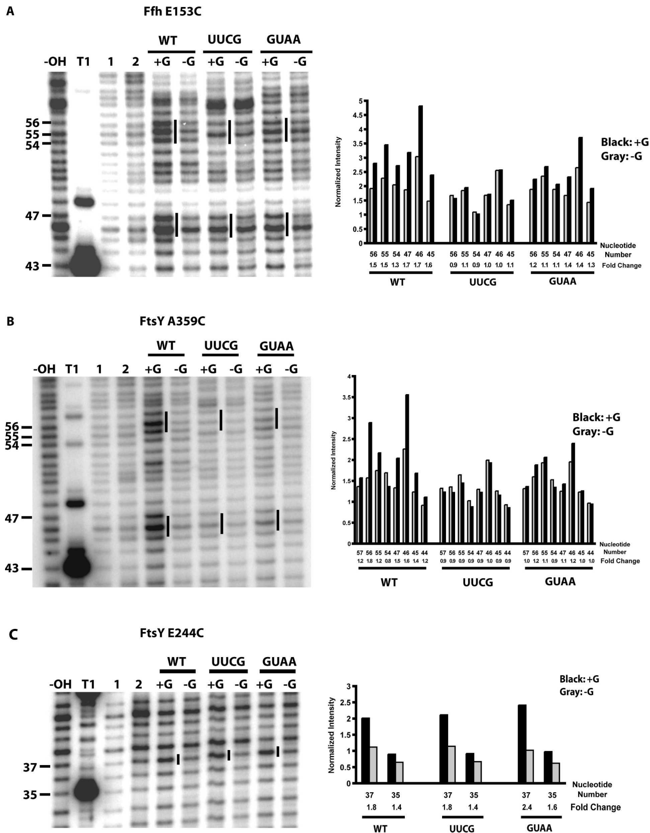
FIGURE 5. Tethered hydroxyl radical probing of SRP-FtsY complexes. Strand scission of full-length wild-type (WT), UUCG, and GUA A 4.5S RNA in a saturable SRP-FtsY complex derivatized by BABE-Fe at positions Ffh E153 (A), FtsY A359 (B), and FtsY E244 (C). Lanes labeled -OH, T1, 1, and 2 indicate 4.5S RNA alkaline hydrolysis, partial T1 RNase guanosine cleavage, 4.5S RNA alone in buffer, or in the presence of cleaving reagents, respectively. Lanes labeled -G and +G indicate the absence and presence of GMPPCP, respectively. Nucleotide positions of 4.5S RNA are indicated on the left. Regions of cleavage sites for wild type and equivalent sites for UUCG and GUA A are indicated by bars. Quantitations of specific nucleotides are shown with normalization for loading differences between the +G and -G lanes for the three RNA constructs. Fold change indicates the intensity of the nucleotide in the +G reaction relative to the -G reaction. These data are representatives of three independent experiments.
