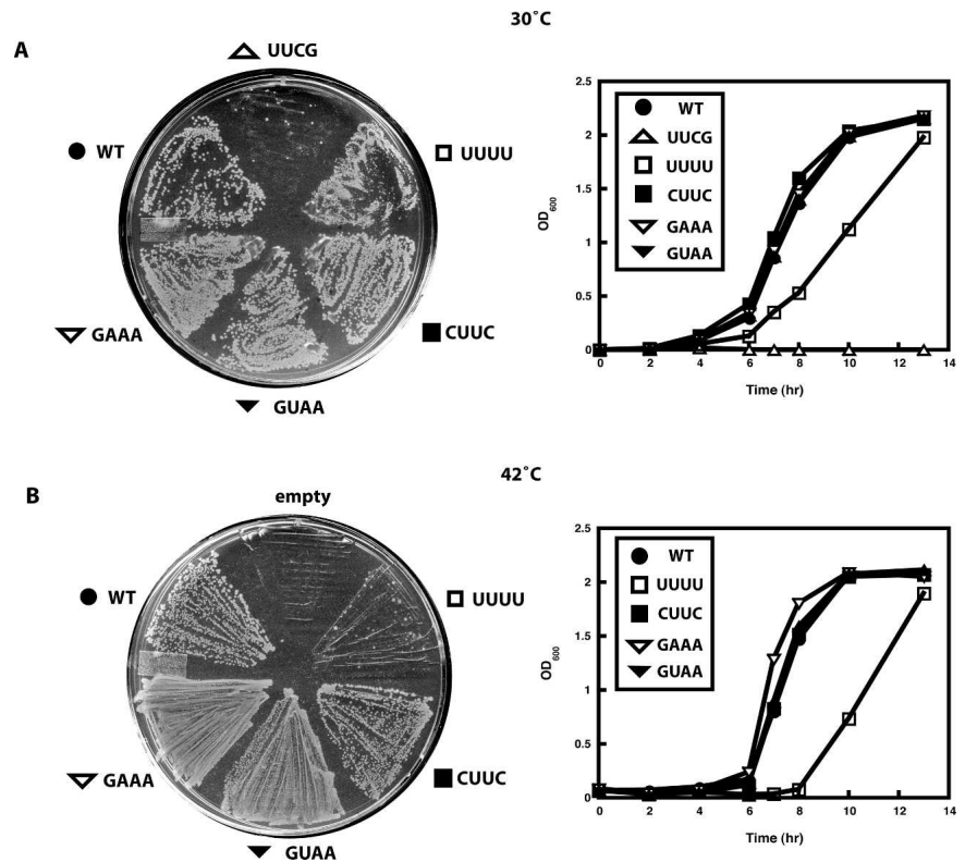
FIGURE 6. In vivo complementation with 4.5S RNA mutants. E. coli strain S1610 transformed with plasmids encoding wild-type (●), UUCG (Δ), CUUC (■), UUUU (□), GUAA (▼), and GAAA (▽) 4.5S RNA were grown at (A) 30°C and (B) 42°C. E. coli transformed with the specified 4.5S RNA construct was streaked onto an agar plate with ampicillin at 30°C. Liquid cultures of the specified 4.5S RNA constructs grown at 30°C were streaked onto an agar plate with ampicillin at 42°C. Growth of the E. coli harboring wild-type, UUCG, UUUU, CUUC, GUAA, and GAAA 4.5S RNA in LB media with ampicillin was monitored over time at the designated temperatures. No data were available for the UUCG mutant at 42°C since there was no growth observed at 30°C. These data are representatives of three independent experiments.
