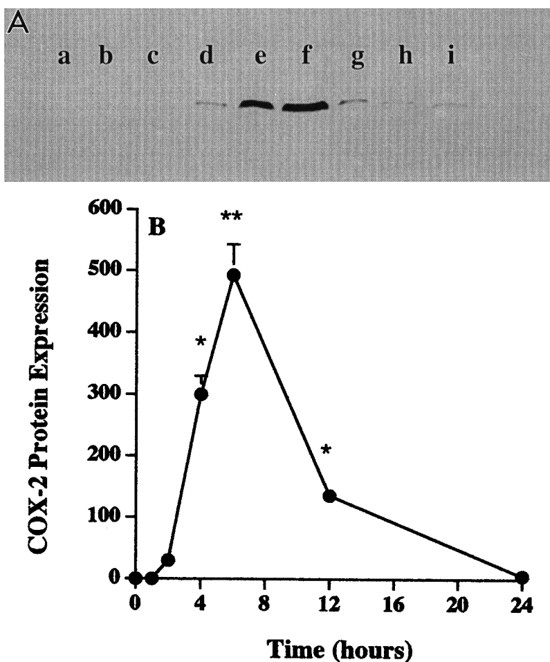
FIG. 6. (A) A representative Western blot (one of three experiments) showing induction of COX-2 (size, 70 kD) protein synthesis by IL-1 \beta for different time periods as follows: lane a, 0 min; lane b, 30 min; lane c, 1 h; lane d, 2 h; lane e, 4 h; lane f, 6 h; lane g, 8 h; lane h, 12 h; and lane i, 24 h. (B) Levels of COX-2 in cells treated with IL-1 \beta (10 ng/ml) for 24 h. * P < 0.05 , ** P < 0.005 ; P value represents the comparison of the effect of IL-1 \beta on COX-2 levels as compared with untreated control. Data are means \pm SE for three separate experiments.
