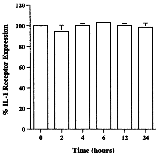
FIG. 3. Levels of IL-1 receptor, type I, in rabbit colonocytes treated with IL-1 (30 ng/ml) for different time periods. No significant increase in the receptor levels was observed at any of the times tested. Data are means±SE for four separate experiments.
