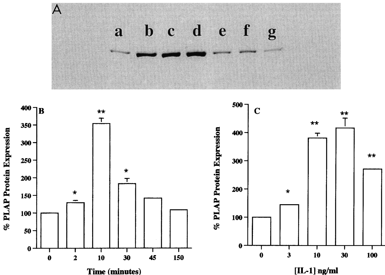
FIG. 4. (A) A representative Western blot (one of four experiments) showing the presence of PLAP (size, 42 kD) and its induction in cells treated with IL-1 (10 ng/ml) for different time periods. Lane a, 0 min; lane b, 2 min; lane c, 10 min; lane d, 30 min; lane e, 1 h; lane f, 12 h; and lane g, 24 h. (B) Levels of PLAP in cells treated with IL-1 (10 ng/ml) for different time periods. (C) Levels of PLAP in cells treated with different concentrations of IL-1 for 10 min. * P < 0.05 , ** P < 0.005 ; P value represents the comparison of the effect of IL-1 on PLAP levels as compared with untreated control. Data are means±SE for four separate experiments.
