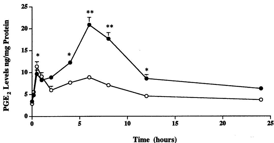
FIG. 8. Levels of PGE 2 in (●) cells treated with IL-1 \beta (10 ng/ml) as compared with (○) cells treated with the IL-1 \beta and COX-2 synthesis inhibitor L-745,337. * P < 0.05 ; P value represents the comparison of the effect of IL-1 \beta on PGE 2 production as compared with COX-2 inhibitor treated cells. Data are means \pm SE for four separate experiments.
