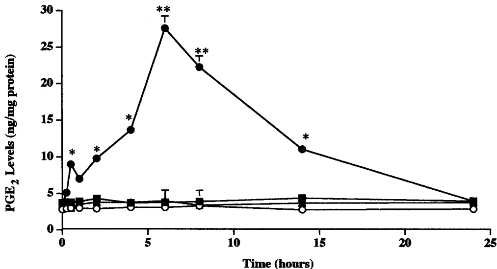
FIG. 7. Levels of PGE 2 in (●) cells treated with IL-1 \beta (10 ng/ml) as compared with (■) control untreated cells, with (○) cells treated with the IL-1ra and with (▲) cells treated with IL-1 \beta and IL-1ra together. * P < 0.05 , ** P < 0.005 ; P value represents the comparison of the treatment on PGE 2 production as compared with untreated time control. Data are means \pm SE for six separate experiments.
