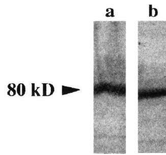
FIG. 1. A representative Western blot (one of three experiments) showing the presence of the IL-1 receptor type I (size, 80 kD) in the cultured colonic epithelial cells (lane a). Lane b shows the presence of the IL-1 receptor in human monocytes as a positive control.
