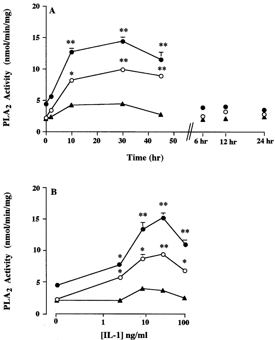
FIG. 5. Activity of total (●), secretory (○), and cytoplasmic PLA 2 (▲): (A) in cells treated with IL-1 (10 ng/ml) for different time periods, and (B) in cells treated with different concentrations of IL-1 for 10 min. * P < 0.05 , ** P < 0.005 ; P value represents the comparison of the effect of IL-1 on PLA 2 levels as compared with untreated control. Data are means \pm SE for six separate experiments.
