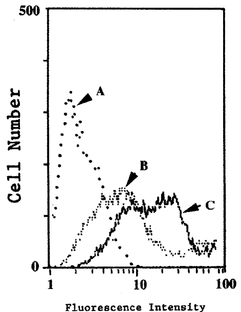
FIG. 2. Single-parameter fluorescence histograms (one of three experiments) of: (A) unstained cells, (B) cells stained with non-immune serum, and (C) cells stained with antibodies against IL-1R type I. There was a significant shift in fluorescence ( P<0.001 ), indicating the presence of the receptor on the epithelial cells.
