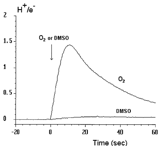
FIG. 6. H^+/e^- ratios measured in medium B for aerobically grown E. coli GO104 ( \Delta cyo ).
