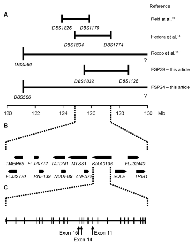
Figure 2. Region spanning the SPG8 locus. A , Markers defining the borders of each described family with the SPG8 mutation and the scaled marker positions on chromosome 8q24.13. B , Candidate region used to search for the SPG8 gene between markers D8S1804 and D8S1774 . Genes in the region are shown in their observed orientation. C , The 28-exon KIAA0196 gene, drawn to scale, with the location of three mutations in exons 11, 14, and 15 highlighted.
