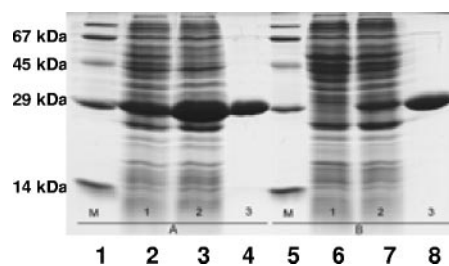
FIG. 2. SDS-PAGE analysis of protein fractions obtained during heterologous expression and purification of His-tagged BamR Geo and BamR Syn . Lanes 1 and 5, molecular mass standards; lanes 2 and 3, insoluble (lane 2) and soluble (lane 3) protein fractions of E. coli cells containing a plasmid with bamR Geo after induction by IPTG; lane 4, His-tagged BamR Geo (approximately 30 kDa) after purification by Ni-chelating affinity chromatography; lanes 6 and 7, soluble proteins of E. coli containing a plasmid with bamR Syn before (lane 6) and after (lane 7) induction by IPTG; lane 8, His-tagged BamR Syn (approximately 30 kDa) after purification by Ni-chelating affinity chromatography. Proteins were visualized by staining with Coomassie blue.
