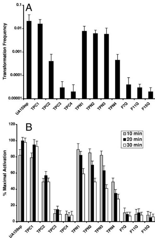
FIG. 6. Effects of truncated peptides or peptides with amino acid substitutions on the activation of quorum sensing for genetic competence. (A) Peptide-dependent induction of genetic competence. (B) Percentages of maximal activation by synthetic peptides. The \beta -Gal activities were assayed in triplicate in two independent experiments.
