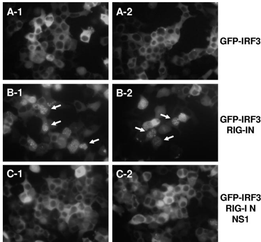
FIG. 4. Inhibition of RIG-IN-induced nuclear translocation of GFP-IRF-3 by NS1. 293T cells were transfected with 250 ng of the pEGFP-IRF-3 expression plasmid in the absence (A) or presence of 250 ng of RIG-IN expression plasmid alone (B) or with 2 \mu g of NS1 expression plasmid (C) as indicated. Nuclear translocation of GFP-IRF-3 was monitored at 48 h posttransfection under a fluorescence microscope. Representative cells with nuclear translocation of GFP-IRF-3 are indicated with arrows. Two representative fields per transfection are shown.
