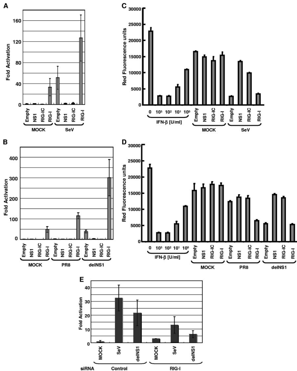
FIG. 7. Involvement of RIG-I in SeV- and influenza A virus-induced IFN- \beta production. (A and B) RIG-IC inhibits activation of IFN- \beta promoter by viral infection. 293T cells were transfected with 0.5 \mu g of pIFN \beta -CAT, 0.5 \mu g of pCAGGS-Luc, and 0.5 \mu g of pCAGGS, pCAGGS-NS1, pCAGGS-Flag-RIG-IC, or pCAGGS-Flag-RIG-I, as indicated, using CaPO 4 . The reporter assays were conducted in triplicate. At 24 h posttransfection, cells were mock infected or infected with SeV, influenza A/PR/8/34 virus, or delNS1 virus at an MOI of 1. Cells were collected at 24 h postinfection and subjected to CAT assays. Relative CAT activity was normalized against relative luciferase activity. The y axis indicates activation ( n -fold) of the IFN- \beta promoter by setting the reporter activities of empty pCAGGS-transfected and mock-infected cells at 1. (C and D) Suppression of virus-induced IFN- \beta production by RIG-IC and NS1. Before cells were collected, culture media were harvested and subjected to a bioassay for determination of IFN levels/production based on RFP expression in NDV-mRFP-infected Vero cells. The y axis indicates the red fluorescence produced by NDV-mRFP. (E) siRNA for RIG-I inhibits activation of IFN- \beta promoter by viral infection. To knock down the expression of RIG-I, RNA interference was performed with siRNA (see Materials and Methods). Expression of RIG-I was downregulated in Stealth_1199-transfected cells but not in Stealth_control_1199-transfected cells (data not shown), and that of \beta -actin was not affected by the transfection of both Stealth_1199 and Stealth_control_1199 (data not shown). After incubation, cells were mock infected or infected with SeV or delNS1. After the infection, cells were incubated for 24 h and then cells were collected and subjected to CAT assay. The y axis indicates activation ( n -fold) of IFN- \beta promoter by setting the reporter activity of Stealth_control_1199 and the reporter plasmid-transfected and mock-infected cells at 1.
