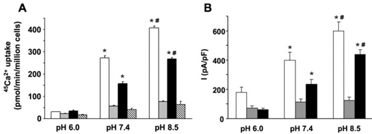
FIG. 5. Functional recovery of TRPV5 activity after chemobleaching is elevated at alkaline pH. (A) ^{45}\text{Ca}^{2+} uptake at different extracellular pH values of MDCK cells stably expressing EGFP-TRPV5 ( n = 6 ). To inhibit TRPV5-mediated ^{45}\text{Ca}^{2+} uptake, 10 \mu\text{M} of ruthenium red was added. The irreversible blocker MTSET ( 5 \text{ mM} ) was applied to study the functional recovery of TRPV5 after MTSET treatment. White bars represent ^{45}\text{Ca}^{2+} uptake under normal conditions, gray bars represent the continuous presence of MTSET, black bars represent recovery after MTSET treatment, and hatched bars represent recovery in the presence of ruthenium red. Significant differences in pH-dependent ^{45}\text{Ca}^{2+} uptake compared to that in MTSET- or ruthenium red-treated cells are indicated by an asterisk ( P < 0.05 ). Significant increases in ^{45}\text{Ca}^{2+} uptake compared to ^{45}\text{Ca}^{2+} uptake at pH 7.4 are indicated by a number symbol ( P < 0.05 ). (B) After 10 min of MTSET pretreatment, whole-cell currents recorded from HEK293 cells transiently transfected with TRPV5 were measured in extracellular solution at the specified pH ( n = 8 ). White bars represent the average current densities in the absence of MTSET, gray bars indicate the average current densities with MTSET continuously present in the extracellular solution, and black bars show the recovered currents after MTSET pretreatment. Asterisks indicate a significant difference ( P < 0.05 ) compared to that for cells continuously treated with MTSET and the number symbol shows a significant difference ( P < 0.05 ) compared to the average current measured in normal extracellular solution (without MTSET) at pH 7.4.
