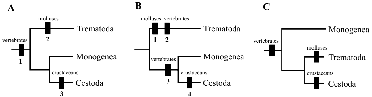
Figure 4 Different views in the interpretations of the host adoption within the neodermatan phylogenetic framework. The relative sequence in the acquisition of invertebrate/vertebrate hosts by three major groups of the Neodermata is illustrated by numerical order (not to scale). (A) 'Vertebrate first' hypothesis; (B) 'Mollusc first' hypothesis (modified [45]); (C) the interpretation of the present study.
