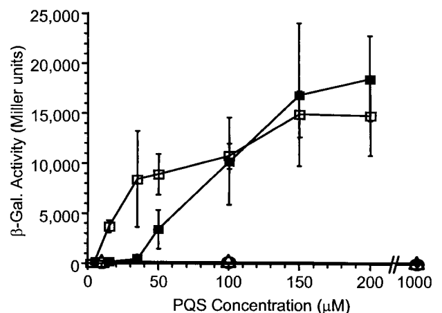
FIG. 6. PQS bioassay with synthetic or natural PQS. Synthetic PQS (open squares), natural PQS (closed squares), 2-hydroxy-3-heptyl-4-quinolone (circles), or 2-heptyl-4-hydroxy-quinoline-N-oxide (triangles) were added to bioassay cultures at the indicated concentrations. Data represent the means of duplicate assays performed during three separate experiments and are presented as \beta -gal activity in Miller units \pm SD n-1 .
