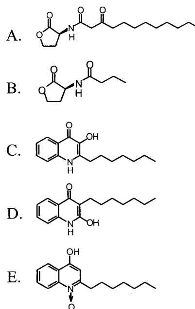
Fig. 1. Chemical structures of relevant compounds. (A) 3-oxo- \text{C}_{12} -HSL. (B) \text{C}_4 -HSL. (C) 2-heptyl-3-hydroxy-4-quinolone (PQS). (D) 2-hydroxy-3-heptyl-4-quinolone. (E) 2-heptyl-4-hydroxy-quinoline- N -oxide.
