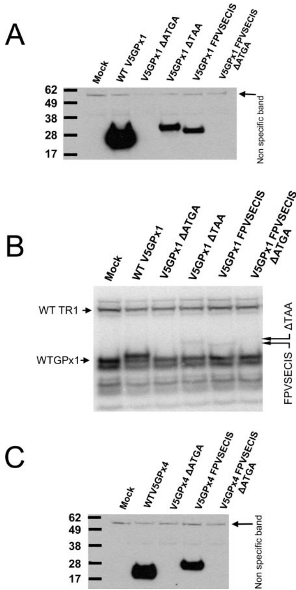
Figure 4. Eukaryotic SECIS elements located in coding regions are functional. (A) Western blot analysis of HEK293 cells transfected with GPx1 constructs containing functional in-frame SECIS elements. The indicated constructs were generated by either deleting the stop codon TAA or replacing the GPx1 3'-UTR with the fowlpox virus SECIS element thereby generating a GPx1-FPV fusion protein. (B) The same samples as shown in A were metabolically labeled with 75 Se and exposed to a PhosphorImager cassette. Location of selenoproteins expressed with the help of coding region SECIS elements is shown by arrows on the right. (C) Western blot analysis of HEK293 cells transfected with GPx4 constructs containing in-frame SECIS elements. GPx4-based constructs were generated by replacing non-homologous sequences with the fowlpox SECIS element thereby generating a GPx4-FPV fusion protein. Lane designations are as follows: Mock, control transfection; WT GPx1, wild-type GPx1 gene; GPx1 ΔATGA, mouse GPx1 gene with disrupted SBP2-binding region; GPx1 ΔTAA, mouse GPx1 gene with its natural stop codon deleted (allowing the ORF to extend beyond the SECIS element which becomes part of the ORF); GPx1 FPV SECIS, the fowlpox SECIS element replacing the 3'-UTR region of the mouse GPx1 gene; GPx1 FPV SECIS ΔATGA, the fowlpox virus SECIS was fused in frame with GPx1 and its SBP2-binding site was disrupted; WT GPx4, cells were transfected with wild-type mouse GPx4 cDNA; GPx4 ΔATGA, the SBP2-binding site in the wild-type GPx4 cDNA was disrupted; GPx4 FPV SECIS, the fowlpox virus SECIS element was fused in frame with GPx4 lacking its own 3'-UTR; GPx4 FPV SECIS ΔATGA, the fowlpox virus SECIS fused to GPx4 was mutated to disrupt the SBP2-binding site.
