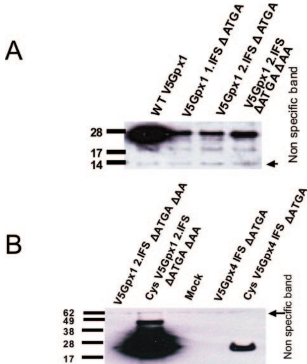
Figure 7. Expression of GPx1 containing a designed in-frame SECIS element. (A) Hepa1-6 cells were transfected with WT GPx1 and different in-frame SECIS element containing constructs. The construct GPx1 2.IFS ΔATGA contains an additional modification in the stem-region as shown in Figure 6A. To disrupt the function of the natural SECIS element, mutations were made in either the SBP2-binding region or the apical loop. (B) Transfection of HEK293 cells. No expression was detectable for GPx4 containing a designed in-frame SECIS element. Note the low expression level of the Cys mutant with the designed in-frame SECIS element compared with GPx1. Expressed proteins were detected by western blot analysis using antibodies specific for V5 tag.
