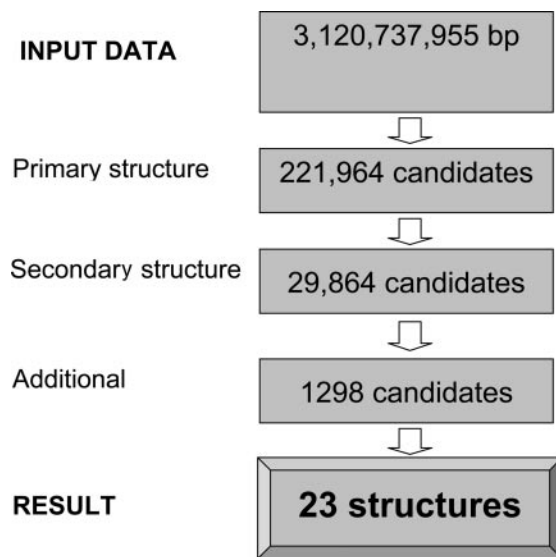
Figure 9. Computational search of the human genome for selenoprotein genes containing SECIS elements in the coding region. A total of 23 selenoprotein genes could be detected using this procedure; however, no additional selenoprotein genes containing SECIS elements in the coding region were found.
