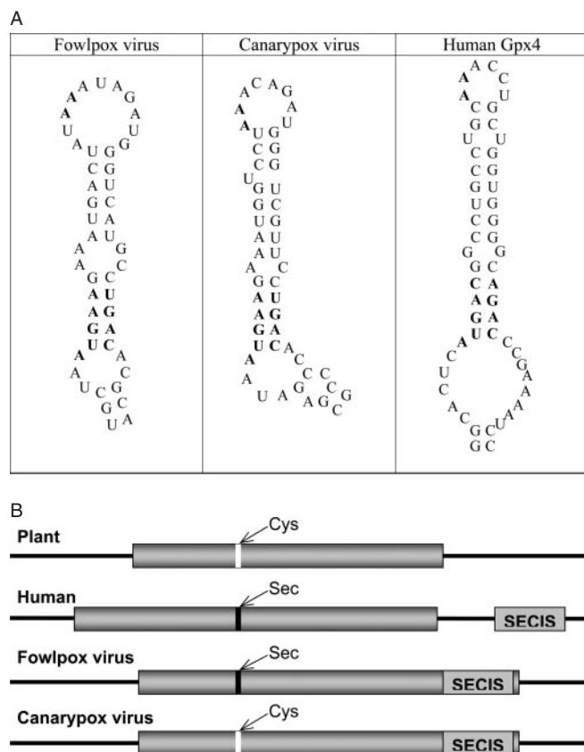
Figure 2. SECIS elements in viral glutathione peroxidases. (A) SECIS structures. Left structure, fowlpox virus GPx4 SECIS element. Middle structure, canarypox virus GPx4 SECIS element. Right structure, H.sapiens GPx4 SECIS element. SECIS core and unpaired AA nucleotides in apical loop are shown in boldface. (B) Location of viral GPx4 SECIS elements within mRNAs and comparison with GPx4 genes from other sources. Cys-containing GPx4 homologs from higher plants lack a SECIS element. In the human Sec-containing GPx4, SECIS element is in the 3'-UTR. In the fowlpox virus Sec-containing GPx4 homolog, SECIS element is in the coding region. In the canarypox virus Cys-containing GPx4, a fossil SECIS element is in the coding region. Location of Cys is shown in white and Sec in black. SECIS elements are indicated by light-gray boxes and ORFs by dark-gray boxes. Left and right black lines represent 5'- and 3'-UTRs, respectively.
