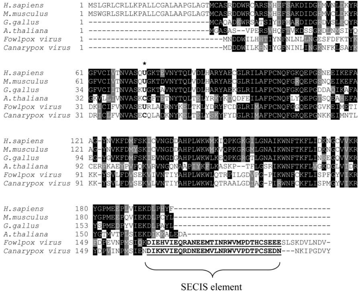
Figure 1. Amino acid sequence alignment of glutathione peroxidases of the GPx4 family. Accession numbers of the sequences used in the alignment are as follows: NP_566128.1 ( Arabidopsis thaliana ), AAH22071.1 ( Homo sapiens ), NP_032188.3 ( Mus musculus ), AAM18080.2 ( Gallus gallus ), AAR83433.1 (canarypox virus), CAE52609.1 (fowlpox virus). In-frame SECIS elements in the C-terminal regions of viral proteins are underlined. Location of catalytic Sec and the corresponding Cys is indicated by an asterisk.
