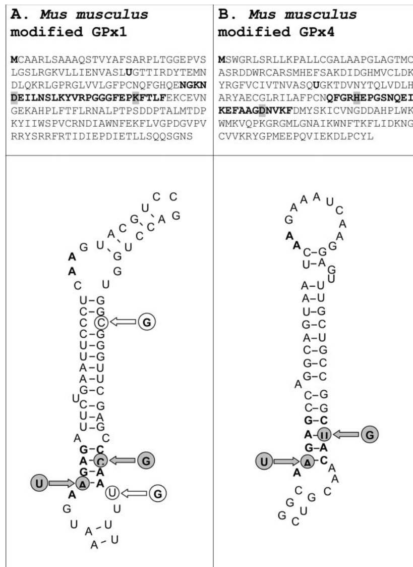
Figure 6. Design of SECIS elements in the coding regions of mammalian selenoprotein genes. (A) Designed GPx1 SECIS element. (B) Designed GPx4 SECIS element. The first amino acids (methionine), Sec, and the SECIS elements are shown in boldface. The amino acids that were mutated to accommodate the designed SECIS elements are highlighted. The newly introduced residues are shown by gray circles, and further changes in the designed GPx1 SECIS are shown by white circles.
