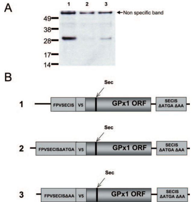
Figure 8. An upstream SECIS element allows readthrough at in-frame UGA codons. (A) Constructs were generated in which the fowlpox SECIS element was cloned upstream and in-frame with the ORF of GPx1 separated by a V5 tag. Control constructs contained mutations in either the SBP2-binding region or in the conserved loop region. (B) Schematic illustration of the constructs used in (A). Numbers on the left correspond to lane designations in A.
