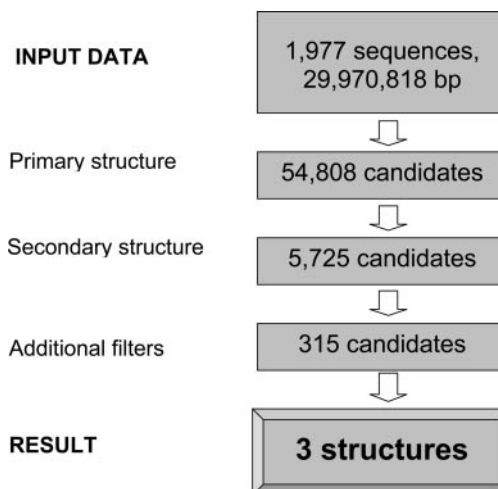
Figure 3. Analysis of viral genomes for selenoprotein genes. Details of the search are provided in Materials and Methods. The search of 1977 viral sequences revealed three SECIS element structures.
