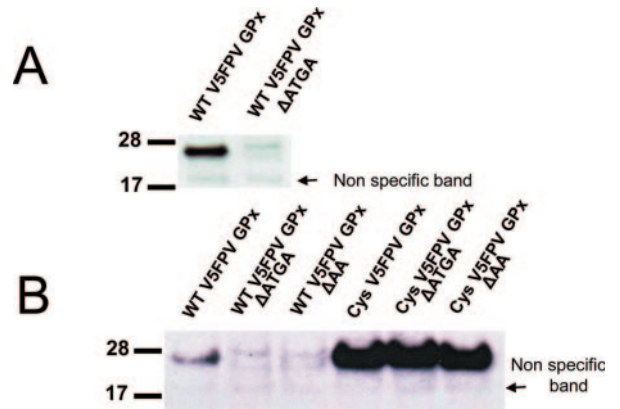
Figure 5. Expression of wild-type fowlpox virus GPx4 in mammalian cell lines. (A) Western blot analysis of mouse hepatoma cell line Hepa1-6 transfected with wild-type fowlpox virus GPx4 construct (WT FPV GPx) or the corresponding construct in which the SBP2-binding site was disrupted (WT FPV GPx ΔATGA). (B) Transfection of HEK293 with wild-type fowlpox virus GPx4 (FPV GPx), its mutants lacking SBP2-binding site (WT FPV GPx ΔATGA) or the conserved AA in the apical loop (WT FPV GPx ΔAA), and the corresponding Sec-to-Cys mutants.
