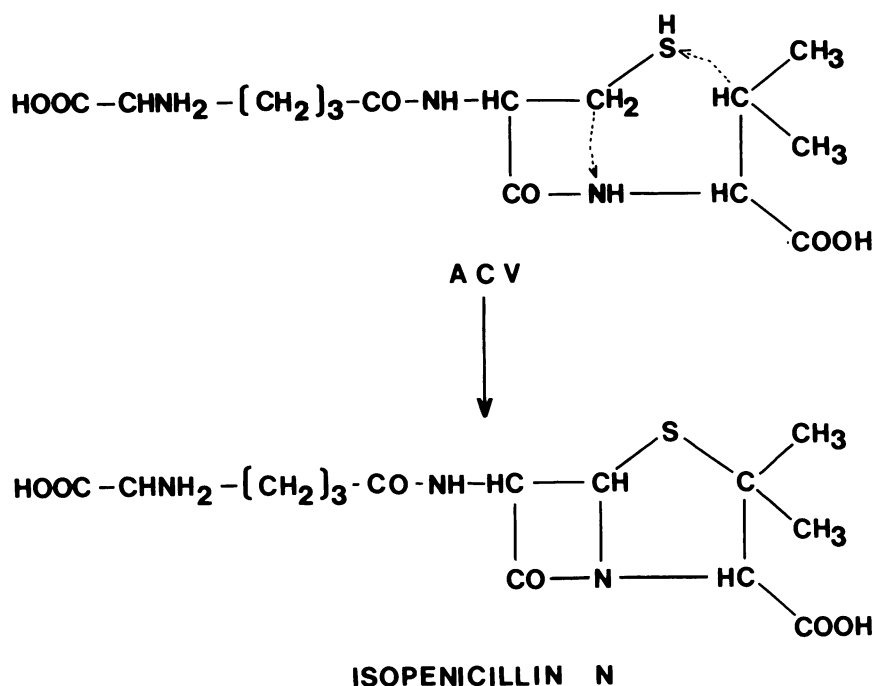
FIG. 1. Cyclization of ACV to isopenicillin N by isopenicillin N synthetase. The dotted arrows indicate the C—N and C—S bonds that are formed during the reaction.
