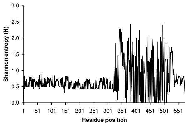
Figure 5 Inter-virus sequence diversity of NP protein.
