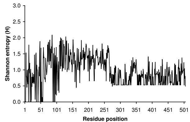
Figure 6 Inter-virus sequence diversity of GPC protein.
