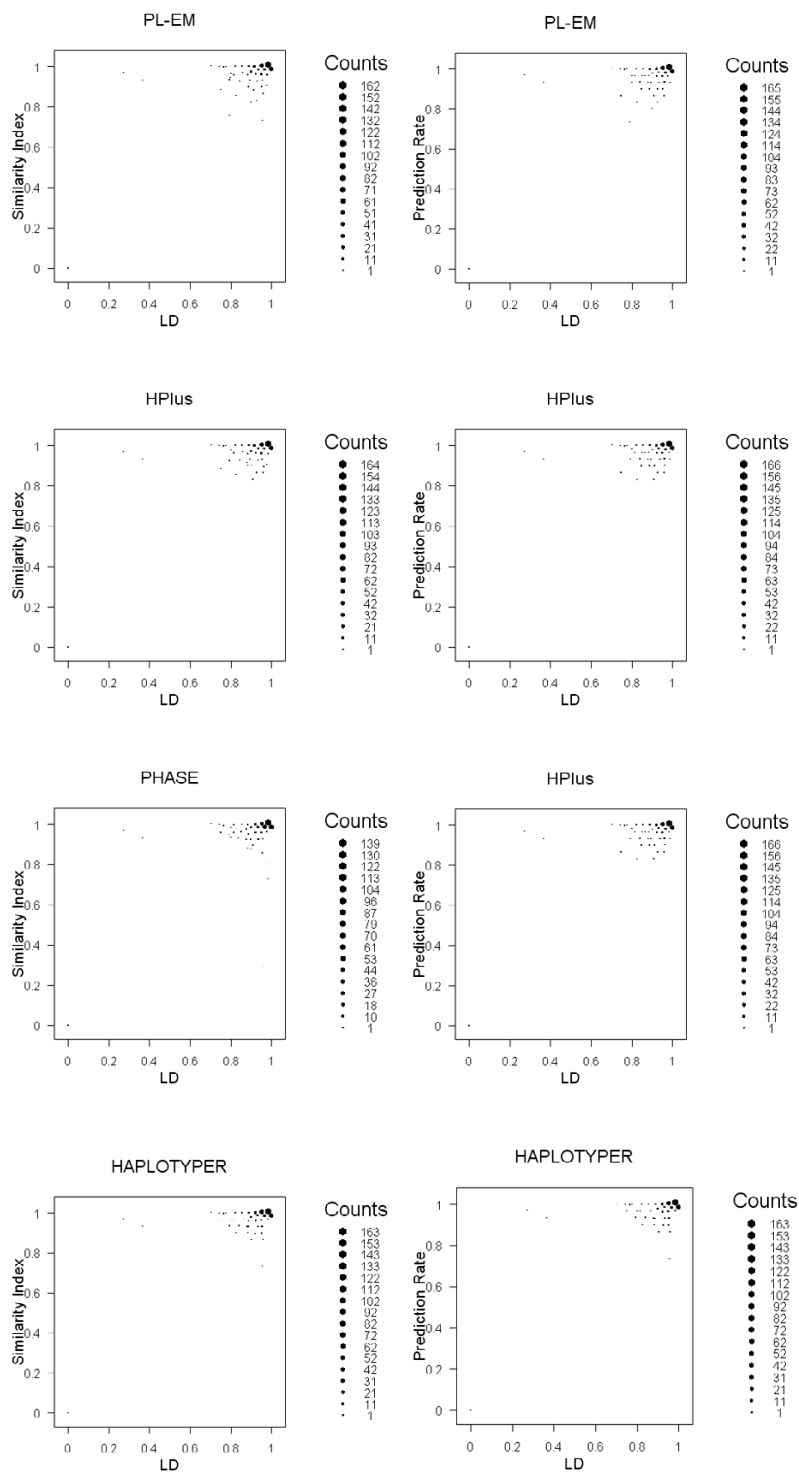
Figure 2 The relationship between the performances of haplotyping methods and the linkage disequilibrium (LD) of the haplotypes within blocks. The plots illustrate for the performances (in similarity Index and Prediction Rate) of empirical methods (PL-EM and HPlus) and Bayesian methods (PHASE and HAPLOTYPER) on analyzing the 500 randomly selected haplotype blocks of the 30 European mothers' genotypes on X-chromosome.
