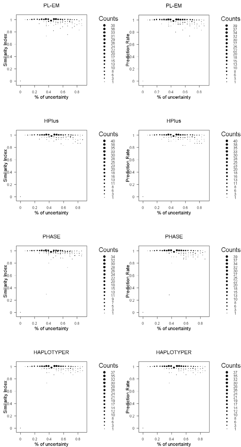
Figure 1 The relationship between the performances of haplotyping methods and the percentage of individuals with uncertainty haplotypes. The plots illustrate for the performances (in similarity Index and Prediction Rate) of empirical methods (PL-EM and HPlus) and Bayesian methods (PHASE and HAPLOTYPER) on analyzing the 500 randomly selected haplo-type blocks of the 30 European mothers' genotypes on X-chromosome.
