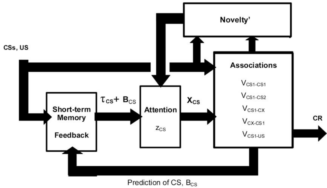
Figure 1. Block diagram of the Schmajuk-Lam-Gray (SLG; 1996) network
