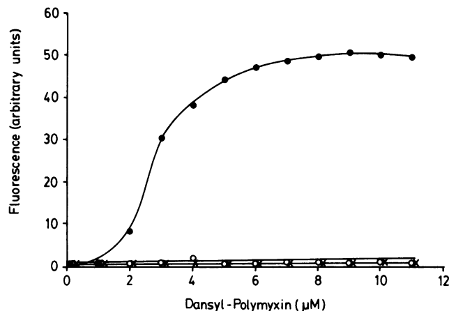
FIG. 1. Binding of dansyl-polymyxin to intact cells. Dansyl-polymyxin was titrated into a cuvette containing 1 ml of 5 mM HEPES buffer (pH 7.35), 10 mM sodium azide, and 20 \mu l of cells which had been centrifuged and suspended in HEPES-azide to an optical density of approximately 1.0 at 600 nm. The fluorescence was recorded as described in Materials and Methods. Symbols: ●, P. aeruginosa H103; ○, P. cepacia ATCC 25609; ×, P. cepacia K61-3.
