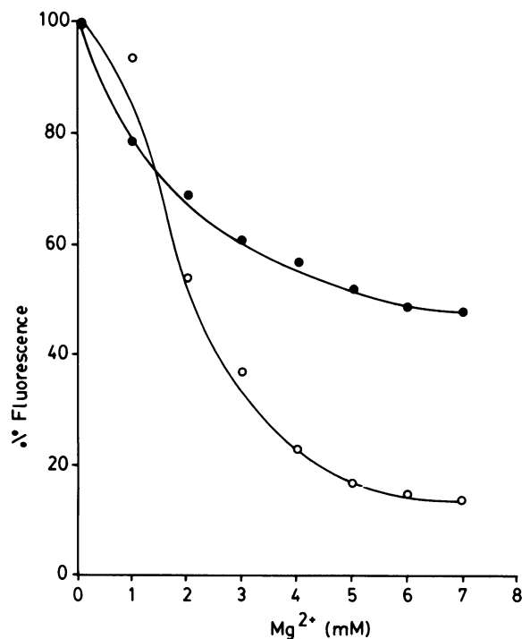
FIG. 3. Inhibition of dansyl-polymyxin binding to LPS by \text{Mg}^{2+} . \text{MgCl}_2 was titrated into a cuvette containing 3 \mu\text{g} of the specified LPS and 2 \mu\text{M} dansyl-polymyxin, and the decrease in fluorescence was recorded. Maximum inhibition was calculated as described in Materials and Methods. Symbols: ●, P. aeruginosa H103; ○, P. cepacia ATCC 25609. Similar data were obtained with other P. cepacia strains.
