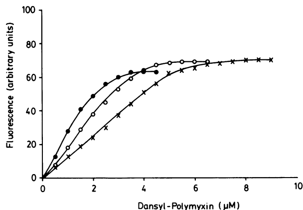
FIG. 2. Binding of dansyl-polymyxin to LPS. Dansyl-polymyxin was titrated into a cuvette containing 1 ml of 5 mM HEPES buffer (pH 7.35) and 3 \mu g of the specified LPS. Symbols: ●, P. aeruginosa H103; ○, P. cepacia ATCC 25609; ×, P. cepacia K61-3.
