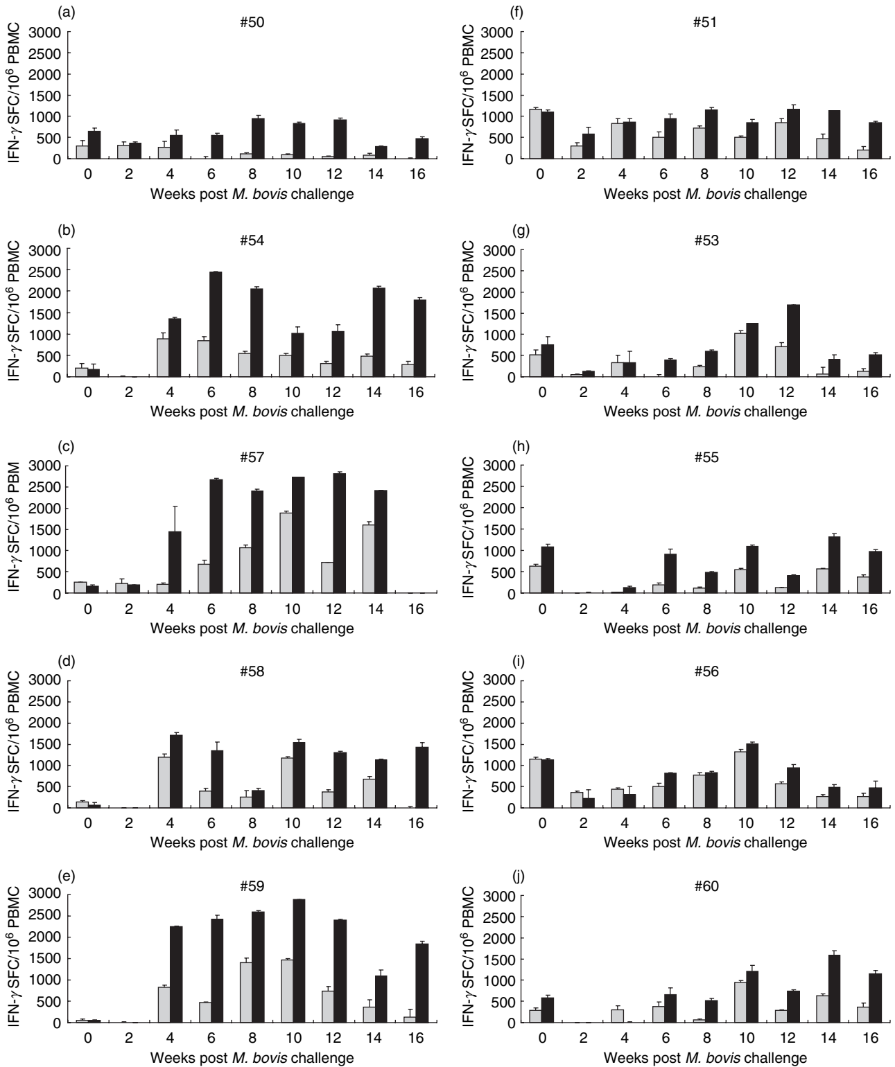
Fig. 3. Detection of post-challenge IFN- \gamma responses by ELISPOT. PBMC from control (a–e) and BCG-vaccinated (f–j) calves were isolated at the indicated time-points post- M. bovis challenge. The number of PPD-A (grey bars)- and PPD-B (black bars)-specific IFN- \gamma SFC was estimated by ELISPOT. The number of SFC obtained by stimulation with medium control was subtracted from the number of SFC observed following antigen stimulation. Results for individual animals are shown.
