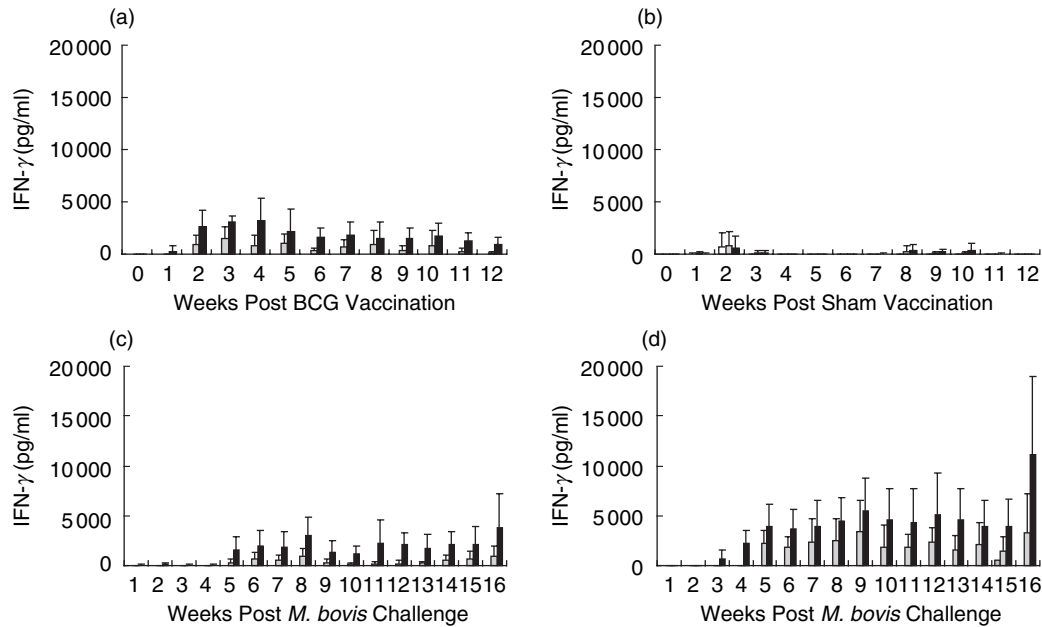
Fig. 1. IFN- \gamma secretion post-BCG vaccination and post- M. bovis challenge. Gnotobiotic calves were vaccinated at 1 day (a) of age with BCG. Control calves (b) were inoculated with medium. Responses were measured for 12 weeks. Subsequently, both BCG-vaccinated calves (c) and control calves (d) were challenged intranasally with M. bovis . Whole blood was stimulated with PPD-A (grey), PPD-B (black) or medium control (white) and IFN- \gamma secretion in supernatants was assessed by ELISA. Means \pm s.d. for groups of five calves are shown.
