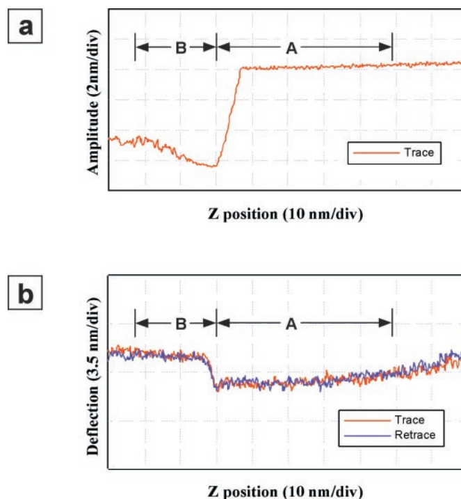
Fig. 3. Force calibration plots for a CVD nanotube tip. (a) Tip amplitude oscillation vs. height above the sample. (b) Tip deflection vs. height above the sample. Regions A and B highlight the pre- and postbuckling areas.
