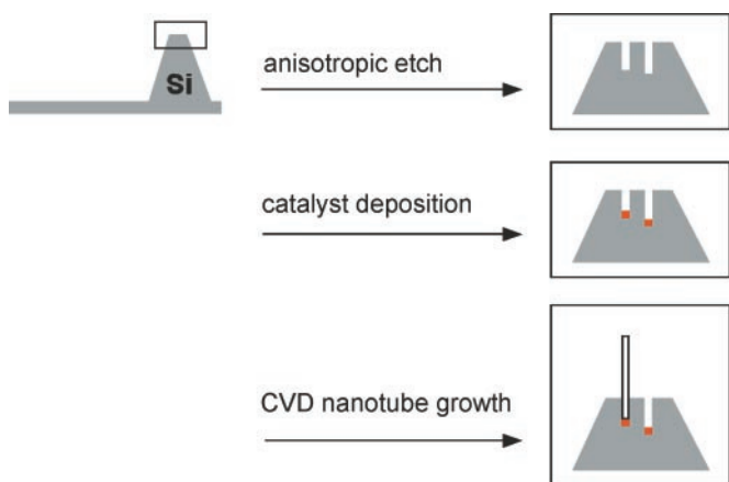
Fig. 1. Schematic of the CVD nanotube tip preparation approach.
