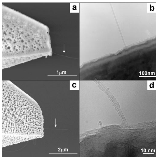
Fig. 2. Electron microscopy of CVD nanotube tips. (a) FE-SEM image of MWNT tubes grown from a Si cantilever/tip assembly. (b) TEM of a CVD MWNT tip. (c) Field emission/SEM image of SWNT bundles grown from a Si cantilever/tip assembly. (d) TEM of several CVD SWNTs comprising a bundle tip.
