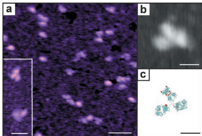
Fig. 4. IgG imaged by a CVD nanotube tip. Large scan area in a shows several molecules that exhibit the characteristic Y shape. ( b ) High resolution images of IgG reveal very little tip-induced broadening when compared with the crystal structure in c . [Bars = 50 nm ( a ), 20 nm ( Inset ), 10 nm ( b ), and 10 nm ( c ).]
