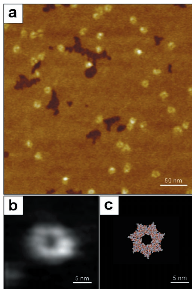
Fig. 5. GroES imaged by a CVD nanotube tip. Large scan area in a shows both “dome” and “pore” conformations, representing the two sides of GroES facing up. ( b ) A higher resolution image of the pore side shows the heptameric symmetry, which matches well with the crystal structure ( c ).
