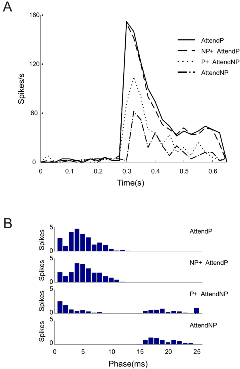
Figure 9. Spiking of the V4 neuron in time to correlated stimulus input. All plots are to excitatory input firing rates of 40 Hz. Preferred input was correlated at the 0 ms phase of oscillation while non-preferred input was correlated at 12 ms phase. Stimulation period is 0.3-0.65 s. (A) The V4 neuron’s response to correlations in the preferred stimulus presented alone with out-of-phase inhibition (Attend P) is represented by the solid black line. Response to preferred and non-preferred stimulus inputs present together with inhibition out-of-phase with the preferred input correlations (NP + Attend P) is depicted by the dashed line. Both stimuli present together with inhibition out-of-phase with non-preferred input correlations (P + Attend NP) is shown by the dotted line, and the dot-dashed line represents response to
