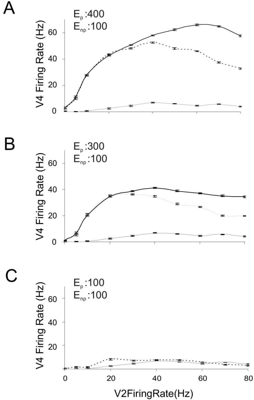
Figure 4. Response of the modeled V4 neuron to pairs of differentially preferred stimuli. The average firing rate response of the V4 neuron to increasing firing rate of the V2 excitatory input is depicted. Response to the preferred stimulus alone (when only V2 E p is active) is in solid black, and to the non-preferred stimulus alone (when only V2 E np is active) is in light gray. Response to both populations being active at equivalent firing rates is represented by the dashed black line. In all cases E np is modeled with 100 excitatory synapses. In (A), (B) and (C) E p has 400, 300 and 100 active synapses respectively. As E p and E np become equally preferred, their responses overlap when activated alone, and hence the solid black line is not visible (C).
