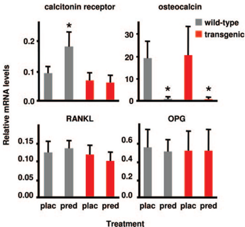
Fig. 3. The TRAP-11 \beta -HSD2 transgene blocked prednisolone stimulation of calcitonin receptor mRNA expression but not inhibition of osteocalcin. Total RNA was extracted from L6 of 6.5-month-old male mice receiving placebo (plac) or prednisolone (pred) for 7 d. Real-time PCR was performed after reverse transcription. Values, relative to that of ChoB, are given as the mean \pm SD (n = 13). *, P < 0.001 vs. placebo.
