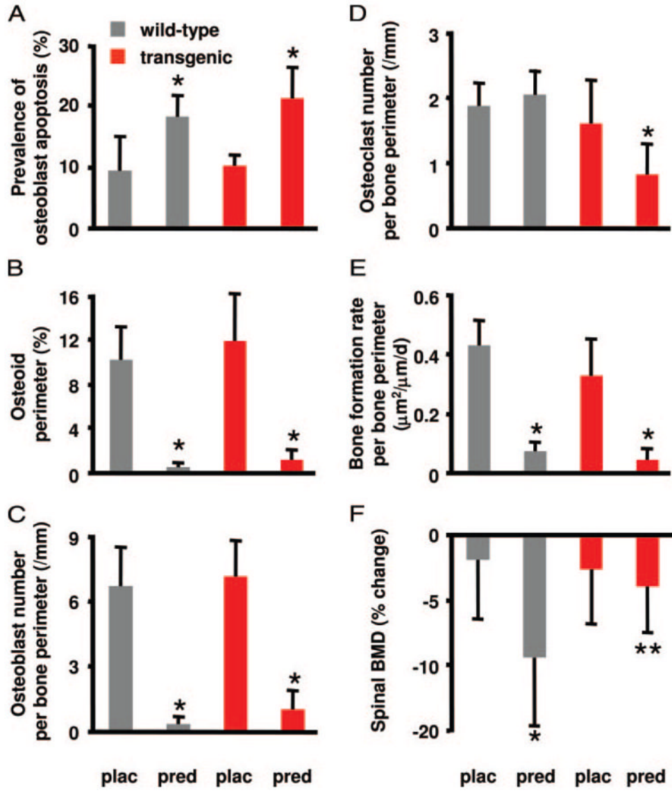
Fig. 4. The TRAP-11 \beta -HSD2 trans-gene prevented the loss of BMD after prednisolone administration. Male wild-type and transgenic mice at 6.5 months of age were given placebo (plac) or prednisolone (pred) pellets for 7 d. A, Prevalence of vertebral cancellous osteoblast apoptosis was evaluated histomorphometrically and values are given as the mean \pm SD (n = 7–12). *, P < 0.001 vs. placebo. B, Osteoid perimeter. C, Osteoblast number per bone perimeter. D, Osteoclast number per bone perimeter. E, Bone formation rate per bone perimeter. Values are given as the mean \pm SD (n = 7–8). *, P < 0.01 vs. wild type. F, Spinal BMD was measured at beginning and end of the experiment. Values, expressed as percent change from the initial BMD, are given as the mean \pm SD (n = 8–12). *, P < 0.001 vs. placebo; **, P < 0.01 vs. wild type.
