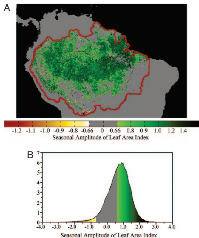
Fig. 2. Seasonal amplitude of LAI. (A) Color-coded map of LAI amplitudes greater than 0.66 or less than -0.66 ; this threshold (0.66) is the smallest LAI difference discernible with the MODIS LAI data set (see SI Materials and Methods ). In regions with dry seasons longer than 3 months, the amplitude is calculated as the difference between the maximum 4-month average LAI in the dry season minus the minimum 4-month average LAI in the wet season. Where the dry season is three or fewer months, the amplitude is calculated as the difference between the dry-season average LAI and the minimum 4-month average LAI in the wet season. The dry and wet seasons are defined based on the precipitation data set at 15' spatial resolution (see SI Materials and Methods ). Thus, the seasons vary spatially and interannually. (B) Distribution of LAI amplitude for all Amazon rainforest pixels. The color scheme is similar to that in A.
