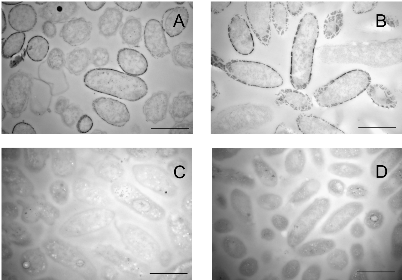
Figure 3 Transmission Electron Microscopy of thin sections of the U(VI) reducing strains DL1 (A and C) and MacA (B and D) before (A, B) and after (C, D) treatment with bicarbonate and air. Bar represents 1 μm
