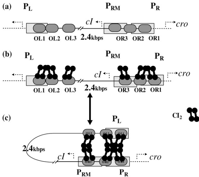
FIGURE 1 \lambda -SWITCH system and the process of O_L participation in the SWITCH. (a) SWITCH is composed of O_R and O_L promoter region and cI , cro genes. O_R region consists of O_{R1} , O_{R2} , and O_{R3} . P_R completely overlaps O_{R1} and partially overlaps O_{R2} , whereas P_{RM} completely overlaps O_{R3} and partially overlaps O_{R2} . (b and c) A schematic picture indicating the transition between unlooping configuration and looping configuration.
