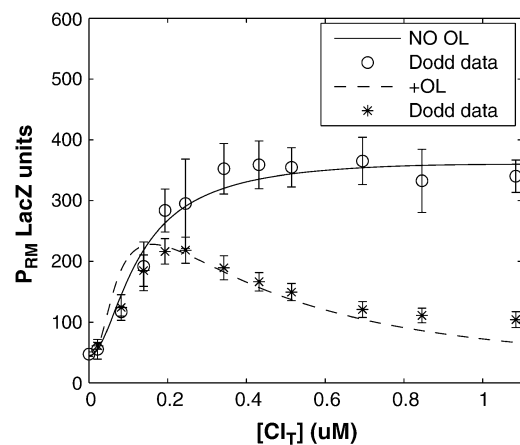
FIGURE 3 P_{RM} activity (LacZ units) versus the total CI concentration for system a (solid line) and system b (dashed line). The experimental data are kindly offered by Dodd et al. (3,4).
