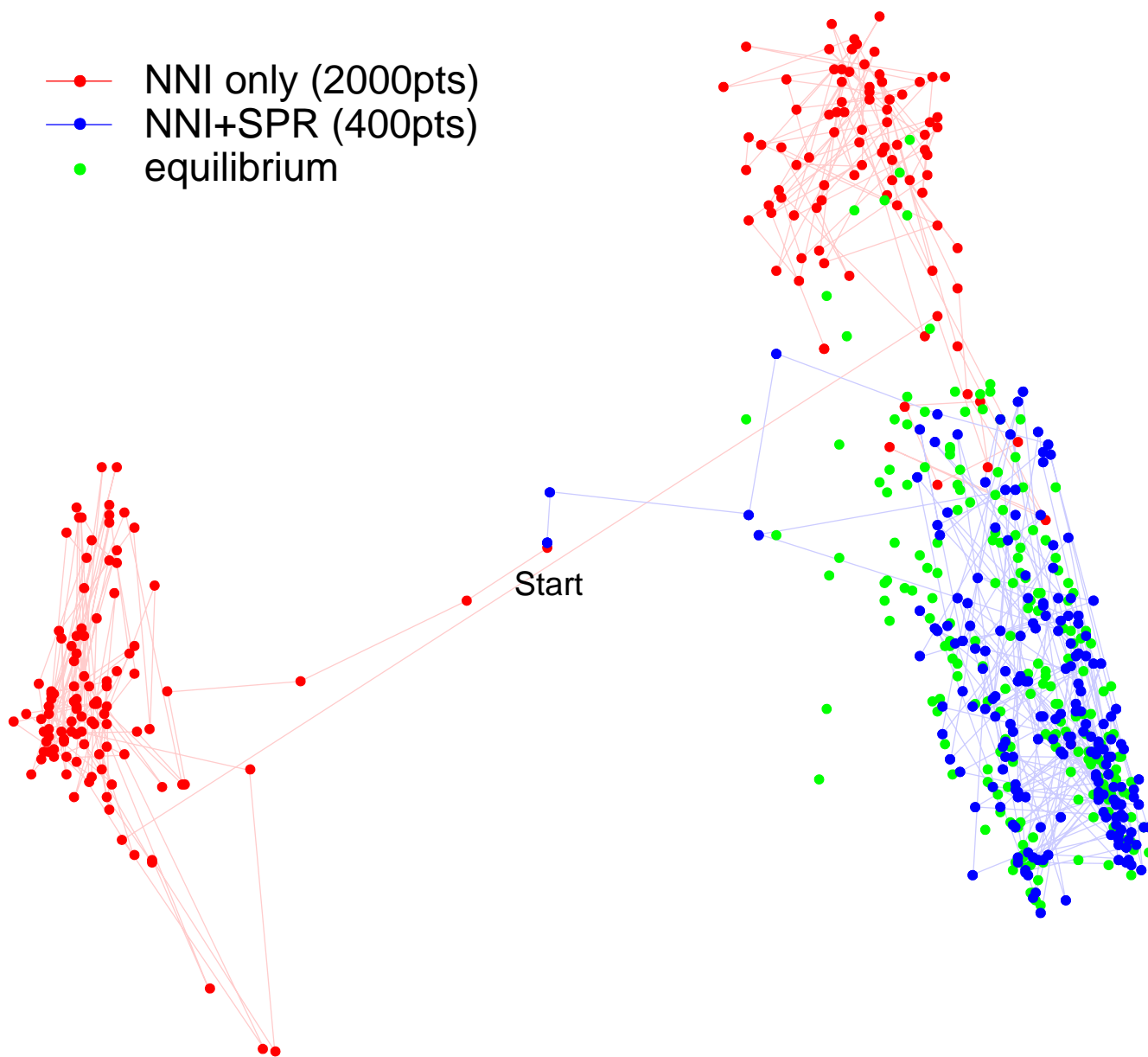
Figure 7 Alignment-aware SPR transition kernel decreases burn-in time. We consider the 27-sequence data set of HIV sequences described in the Results section as Example 2. Points represent 200 topologies sampled from a Markov chains with the alignment-aware SPR transition kernel disabled (red; NNI-only) or enabled (blue; NNI+SPR) or from the equilibrium distribution (green). While the convergence time for Markov chains varies widely, this example illustrates the median convergence time. The NNI-only chain takes 2112 iterations to converge versus only 66 iterations for the NNI+SPR chain. Because the convergence times are so different, the figure depicts every 10th tree for the first 2000 iterations, whereas for the NNI+SPR chain the figure depicts every 2nd tree for the first 400 iterations. Points represent trees projected onto the plane using multidimensional scaling based on the Robinson-Foulds distance. This distance depends only on the topology, not the branch lengths.
