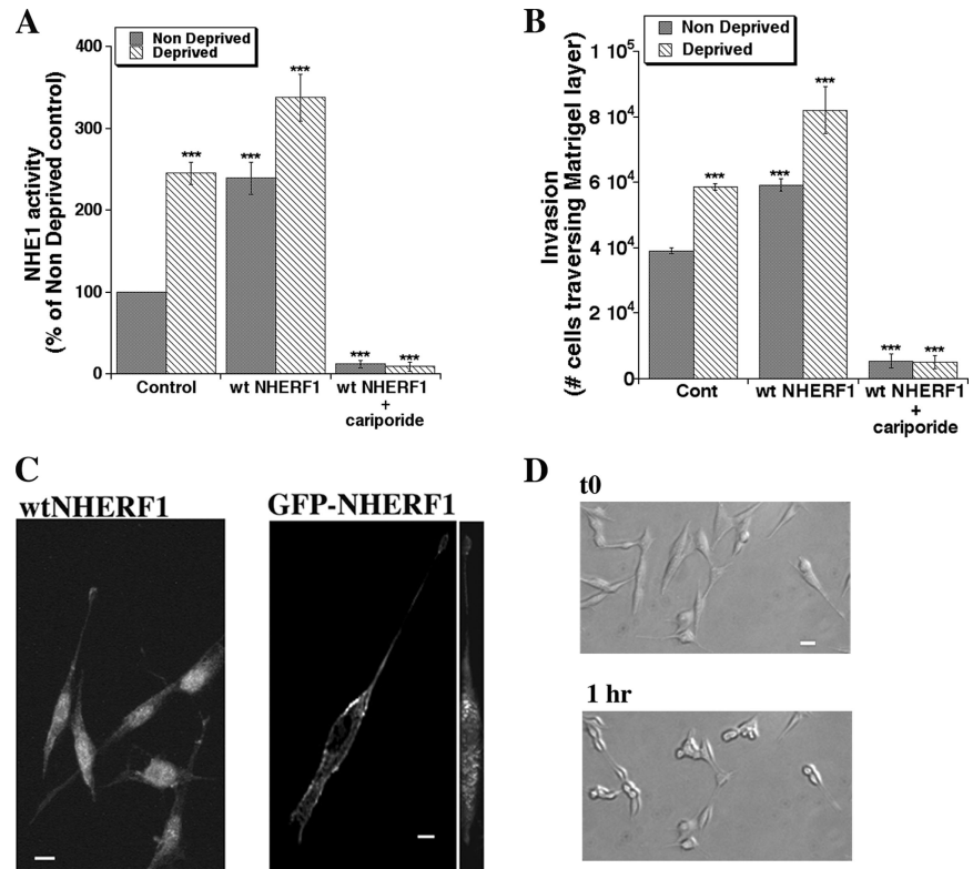
Figure 5. Effect of exogenous NHERF1 overexpression on NHE1 activity and NHE1-dependent invasion, cellular morphology, and pseudopodial protrusion. (A) Transfection of wtNHERF1 (wt) in the pcDNA3.1hygro expression vector increased \text{Na}^+/\text{H}^+ exchanger activity in nonserum-deprived (solid bars) conditions and potentiated the serum deprivation-dependent stimulation (striped bars) of \text{Na}^+/\text{H}^+ exchanger activity. Both basal and NHERF1 overexpressed-dependent activity were >90% inhibited by the benzoylguanidine derivative cariporide (HOE642; 2 \mu\text{M} ). (B) Transfection of wtNHERF1 increased invasive activity in nonserum-deprived conditions (solid bars) and potentiated the serum deprivation-dependent stimulation of invasion (striped bars). Both basal and NHERF1 overexpressed-dependent invasion were >90% inhibited by 2 \mu\text{M} cariporide, demonstrating that NHE1 is the principle mechanism underlying invasion. Error bars are mean \pm SE from five independent experiments performed in quintuplicate. (C) Transfection of either wtNHERF1 or wtGFP-tagged NHERF1 elongated the cells to form a leading edge pseudopodia and redistributed NHERF1 expression to the tip of these pseudopodia. NHERF1 was visualized by immunofluorescence microscopy with anti-NHERF1 or by GFP fluorescence microscopy. Bars, 10 \mu\text{m} . (D) Light transmission images of wtNHERF1-transfected cells treated with 2 \mu\text{M} cariporide at time zero (t0, top) and after 60 min at 100 \times . Bar, 10 \mu\text{m} .
