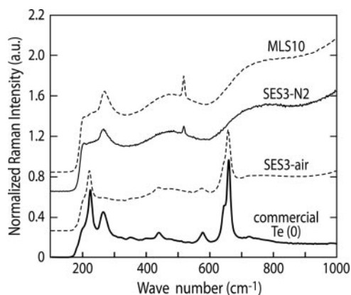
FIG. 7. Raman spectra of purified Te(0) nanomaterials from B. selenitireducens (MLS10), S. barnesii (SES3), and samples from S. barnesii that were exposed to air for over a year compared with those of samples of commercially obtained Te(0). The peak at wave number 270 corresponds to Te(0), while other peaks between 200 and 800 correspond to TeO 2 , with the exception of a peak at 520 corresponding to Si. a.u., arbitrary units.
