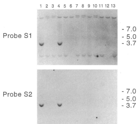
Figure 7. Specific detection of the 3.7-kb allele of VH26 by genomic hybridization. A companion gel to that shown in Fig. 2 (prepared simultaneously with DNA aliquots from the same restriction digests) was sequentially hybridized with oligo probes S1 (above) and S2 (below), which target, respectively, 5' CDR2 and mid-CDR2 of the locus B allele cloned from a 3.7-kb TaqI restriction fragment. For each probe, TMAcI postwash temperature was 57°C, and film exposure time was 7 d. Restriction fragment sizes, in kb, appear to the right.
